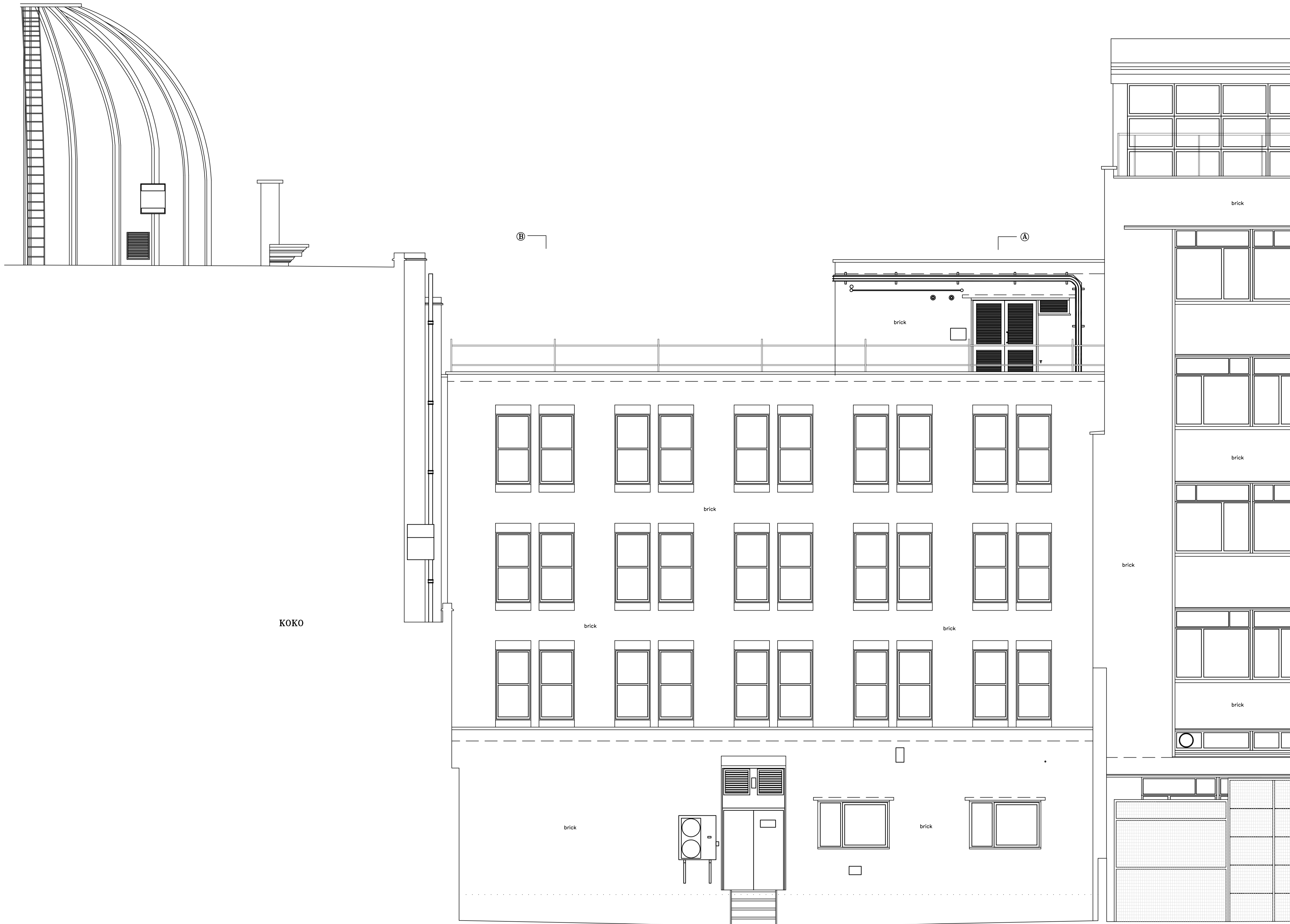
NORTH EAST ELEVATION (BAYHAM PLACE) \Delta 22.00m A.O.D.
