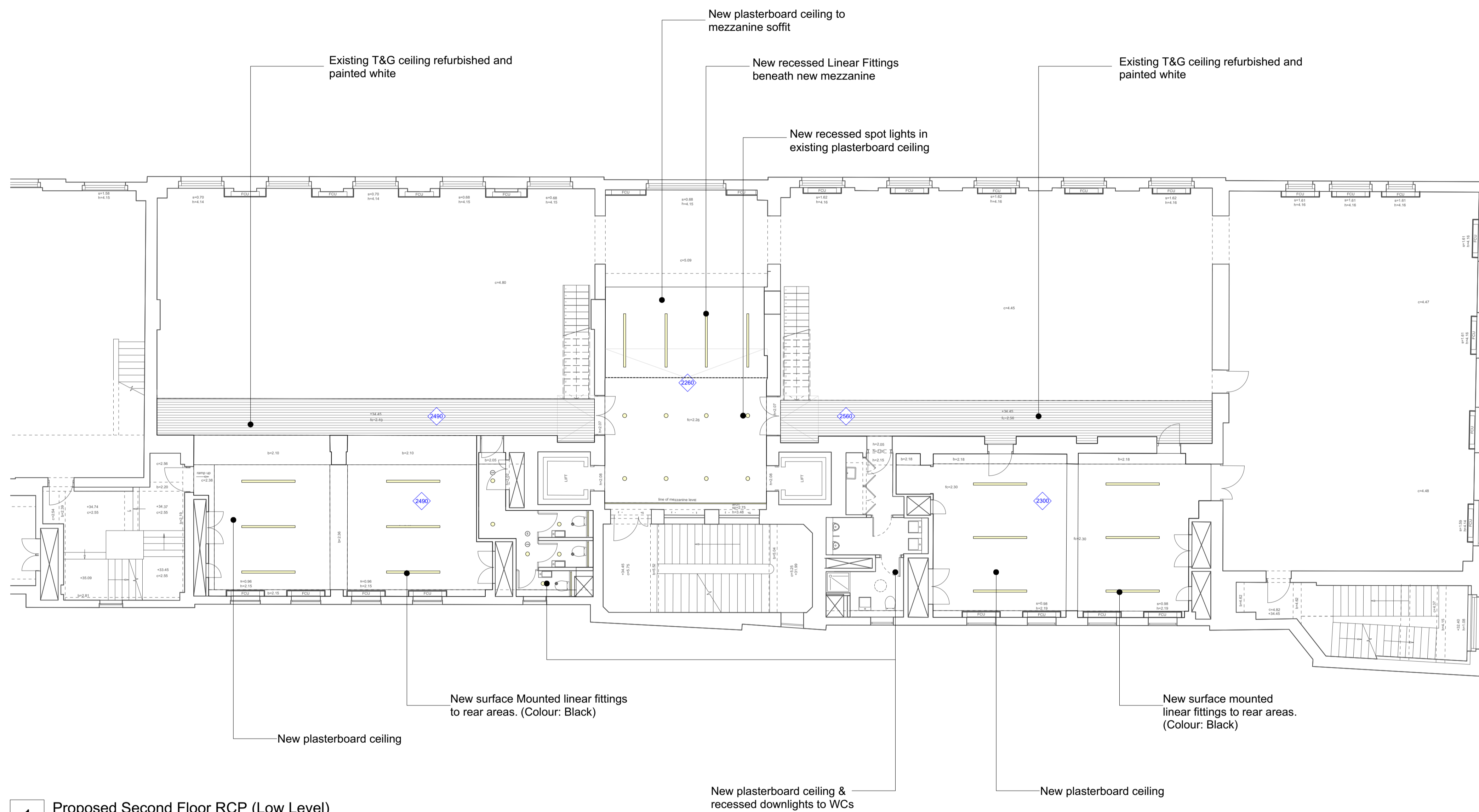
1 Proposed Second Floor RCP (Low Level) Scale: 1:100
