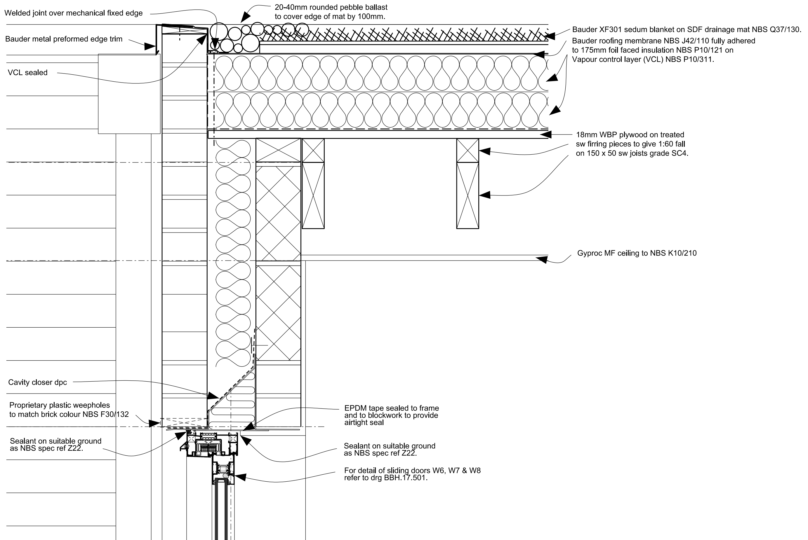
DETAIL 1/610 HEAD OF SLIDING DOOR W6, W7 & W8.
