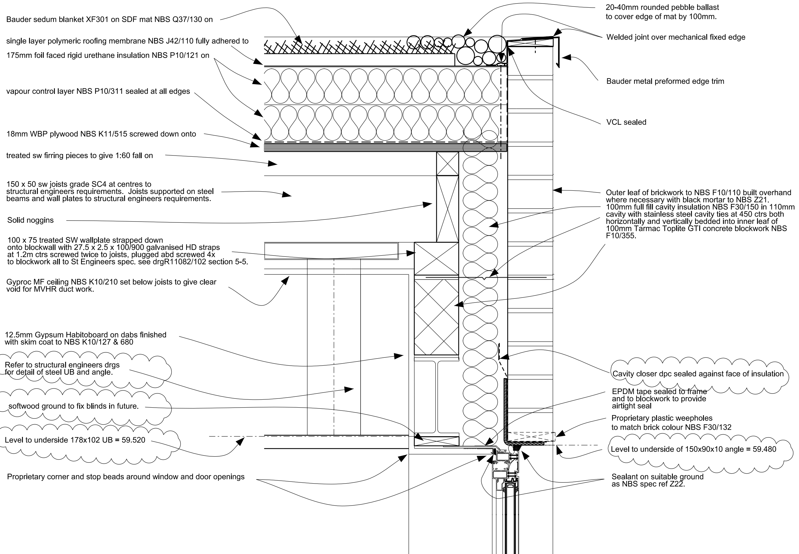
DETAIL 1/603 - SECTION THRO HEAD OF KITCHEN WINDOW
