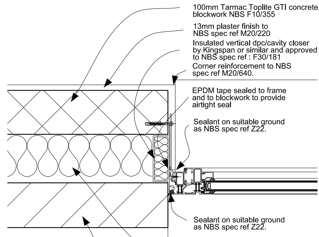
DETAIL 1/411
