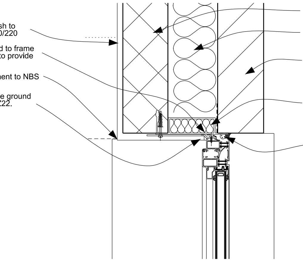
DETAIL 3/411
