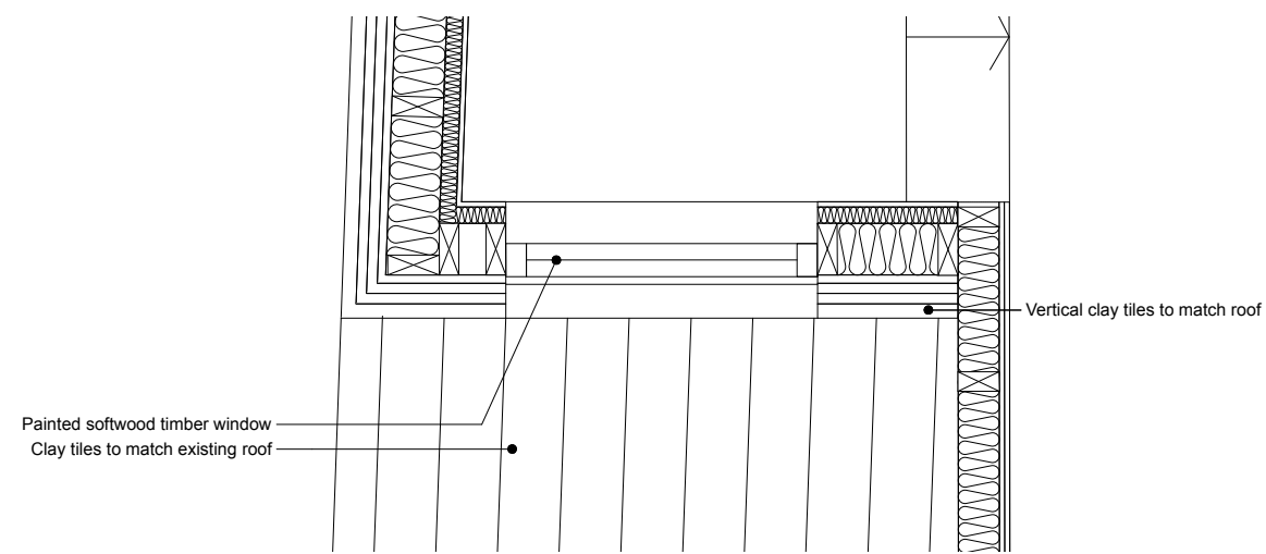
Proposed Window Plan Detail
