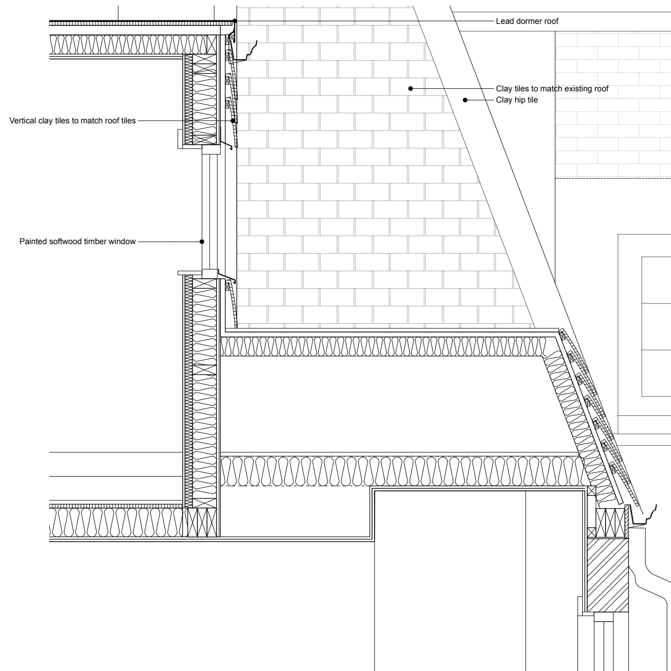
Proposed Window Section Detail
