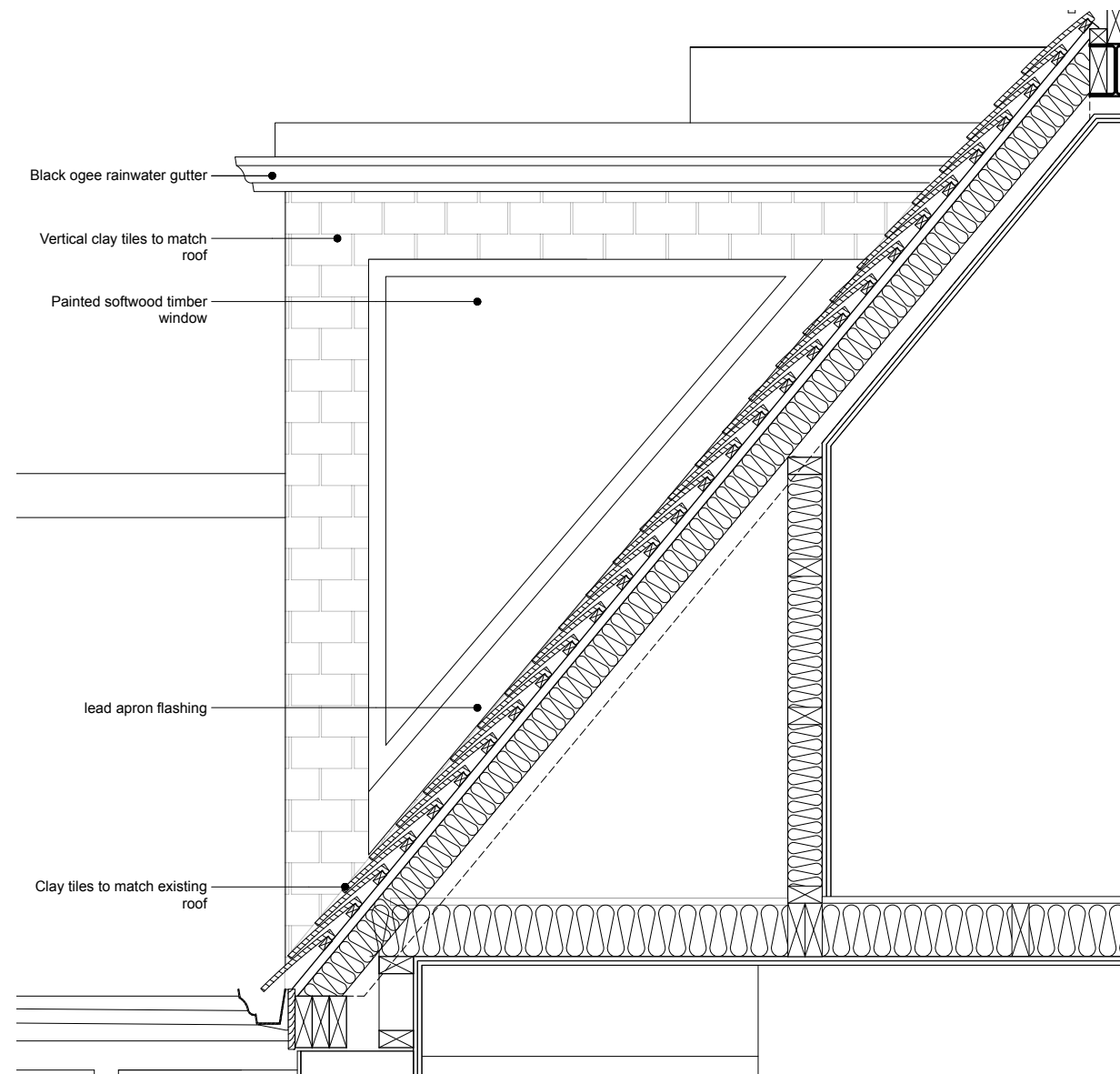
Proposed Window Elevation
