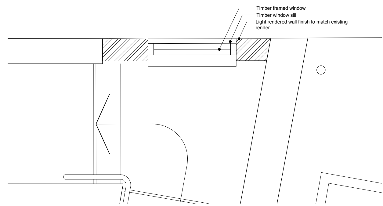
Proposed Window Plan Detail
