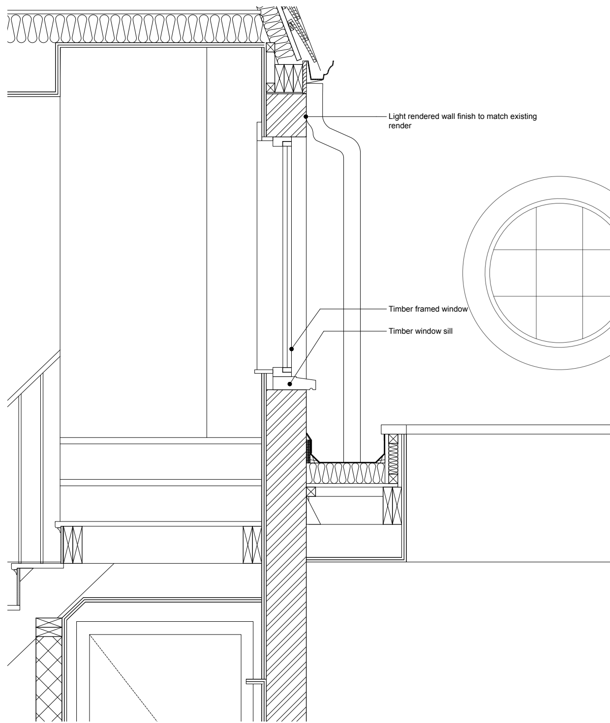
Proposed Window Section Detail
