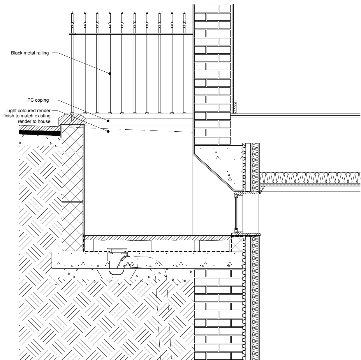
Proposed Lightwell Section Detail
