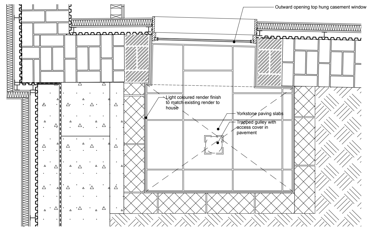
Proposed Lightwell Plan Detail
