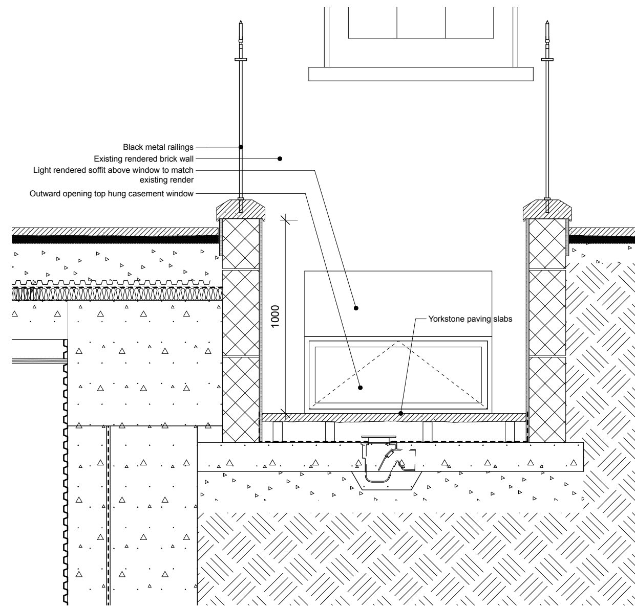
Proposed Lightwell Elevation
