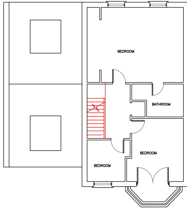
SECOND FLOOR PLAN AS EXISTING
