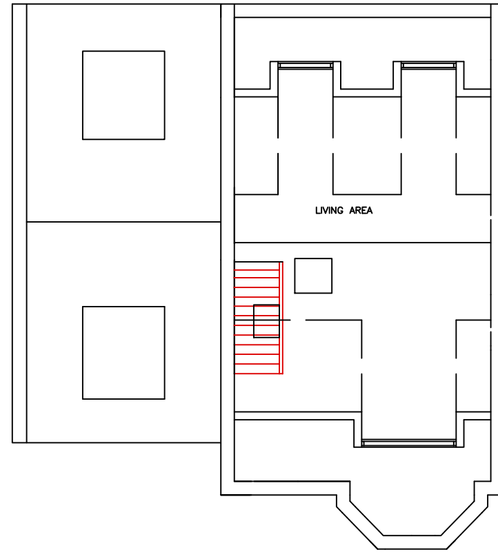
THIRD FLOOR PLAN AS EXISTING
