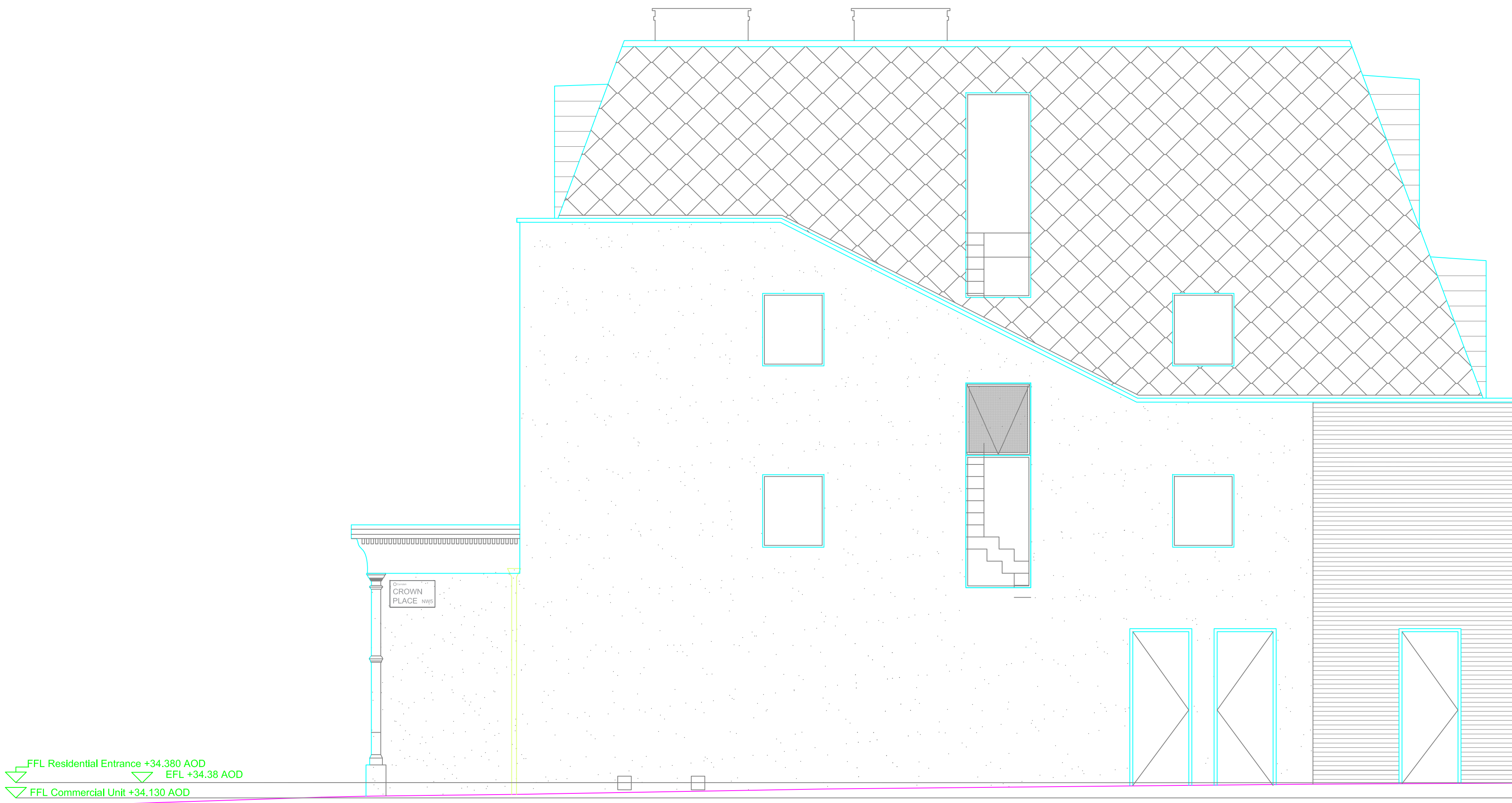
Elevation 4-4 - External right wall Scale 1:50 @ A1
