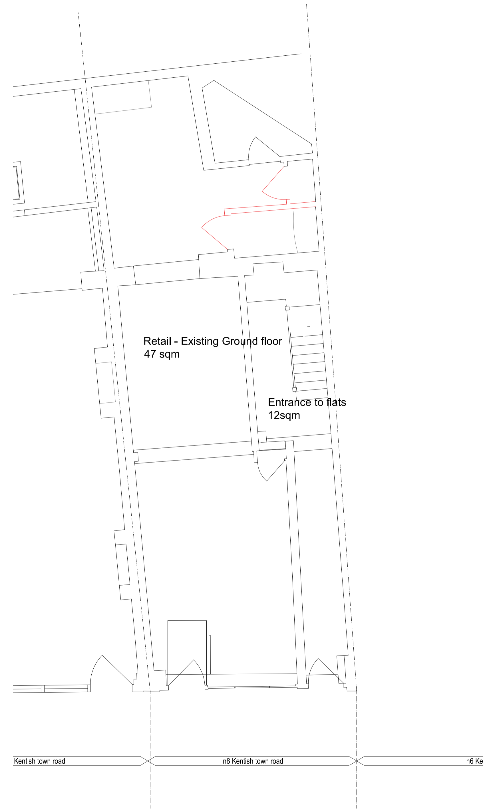
00 Ground floor plan
