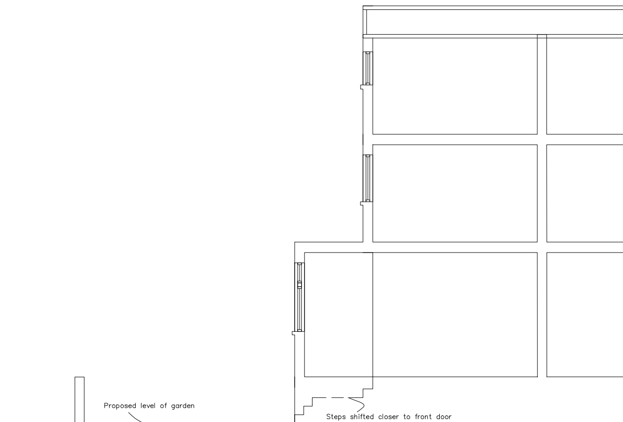
PROPOSED SECTION 1:100
