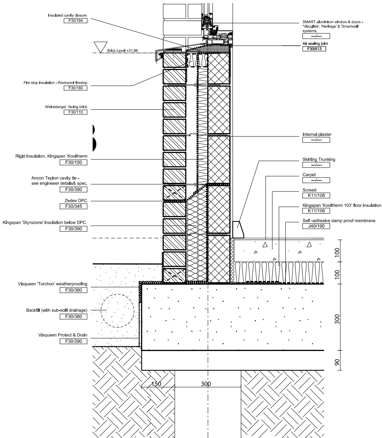
1 Typical Ground detail 1:5 @ A1
