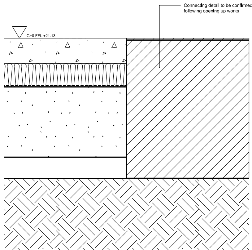
2 Connecting Ground detail 1:5 @ A1
