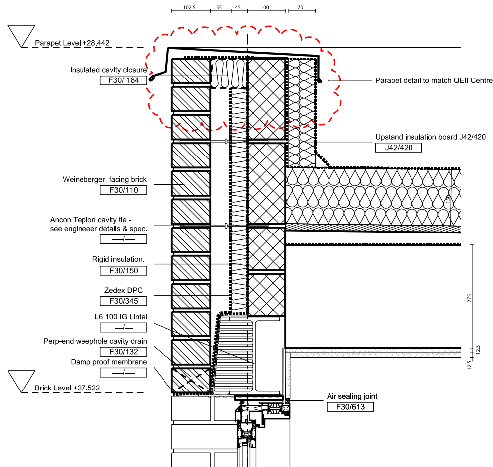
1 Parapet and window section detail 1:5 @ A1
