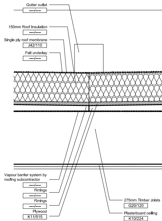
2 Gutter outlet / Roof section Detail 1:5 @ A1
