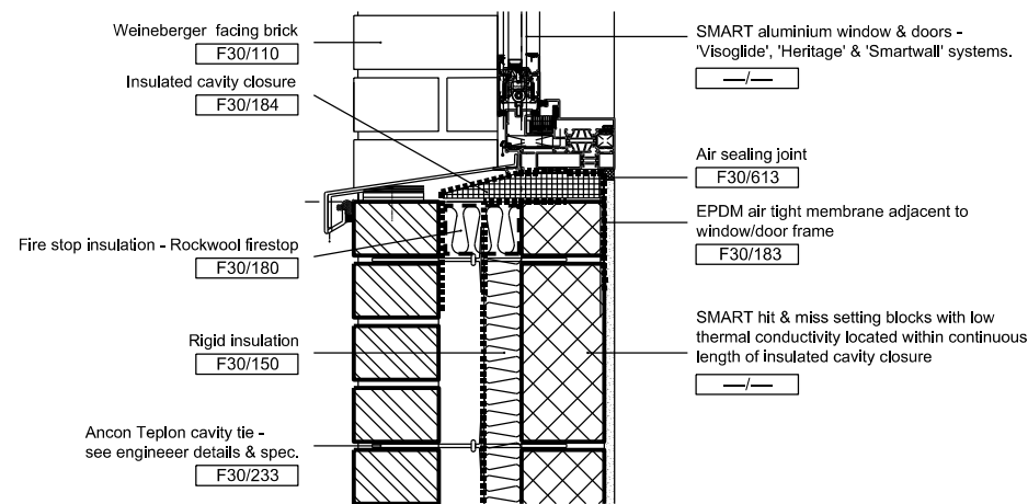
4 Typical window cill detail 1:5 @ A1
