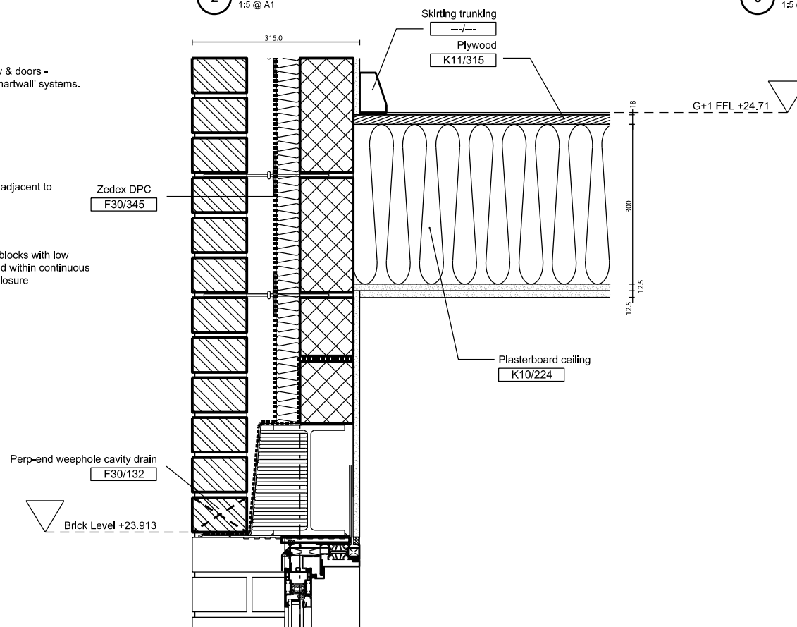
5 Floor to wall and window opening section detail 1:5 @ A1
