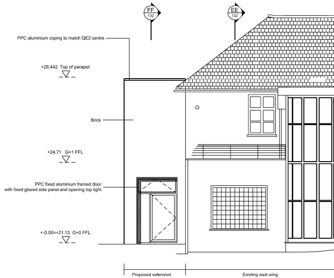
1 Proposed North West Elevation 1:50 @ A1
