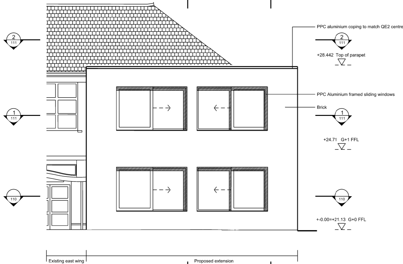
3 Proposed South East Elevation 1:50 @ A1
