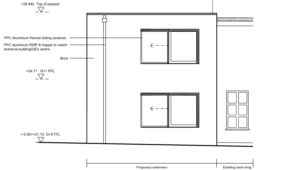
2 Proposed North East Elevation 1:50 @ A1
