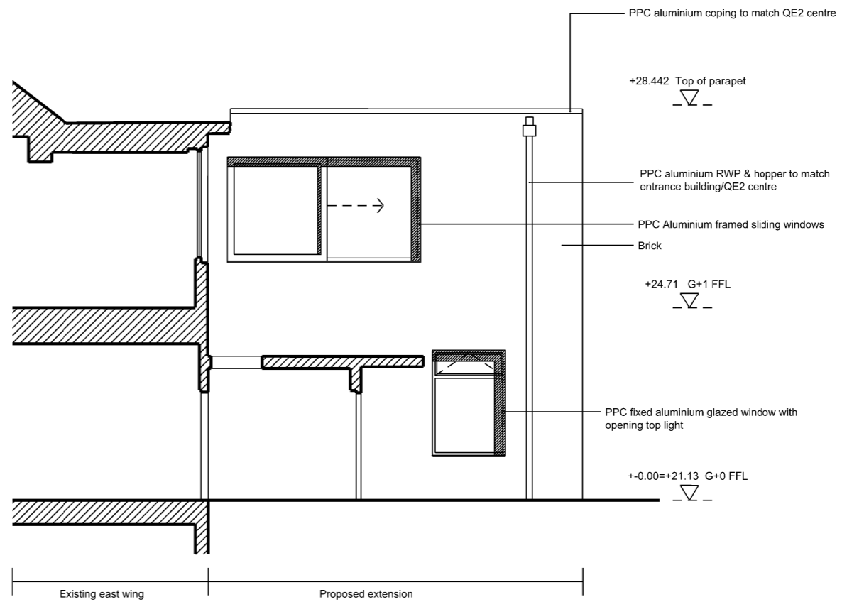
4 Proposed South West Elevation 1:50 @ A1
