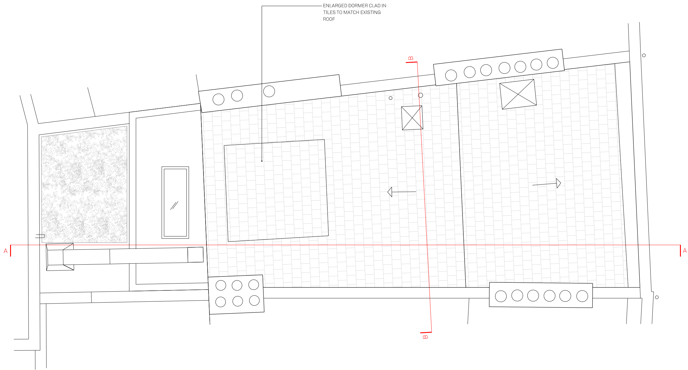
01 PLAN - PROPOSED ROOF PLAN SCALE 1:50
