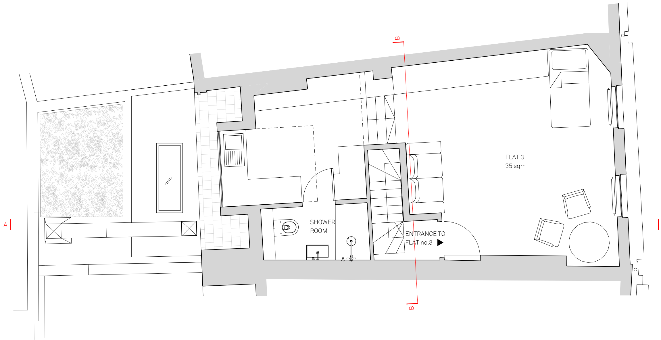
01 PLAN - PROPOSED THIRD FLOOR SCALE 1:50
