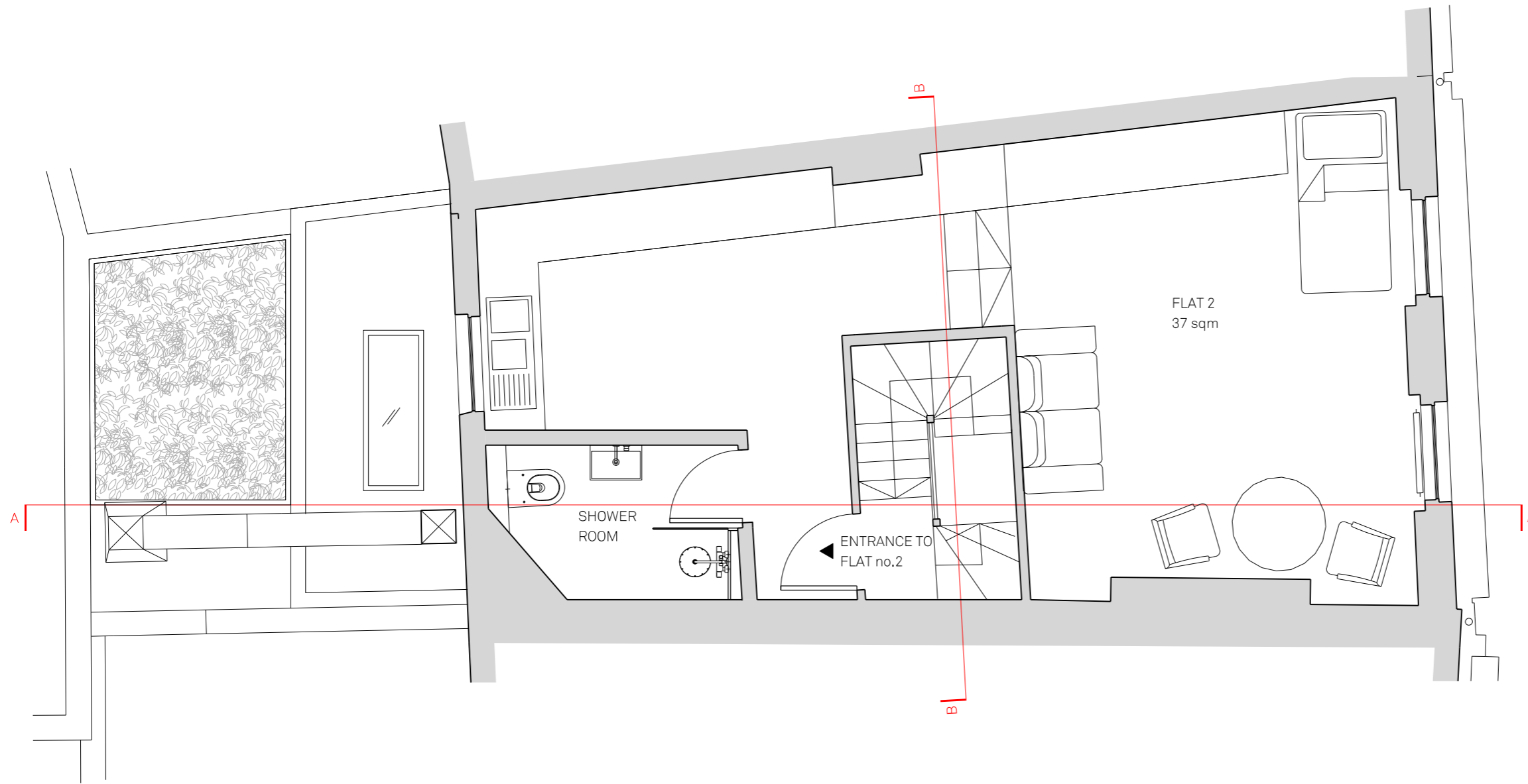
01 PLAN - PROPOSED SECOND FLOOR SCALE 1:50
