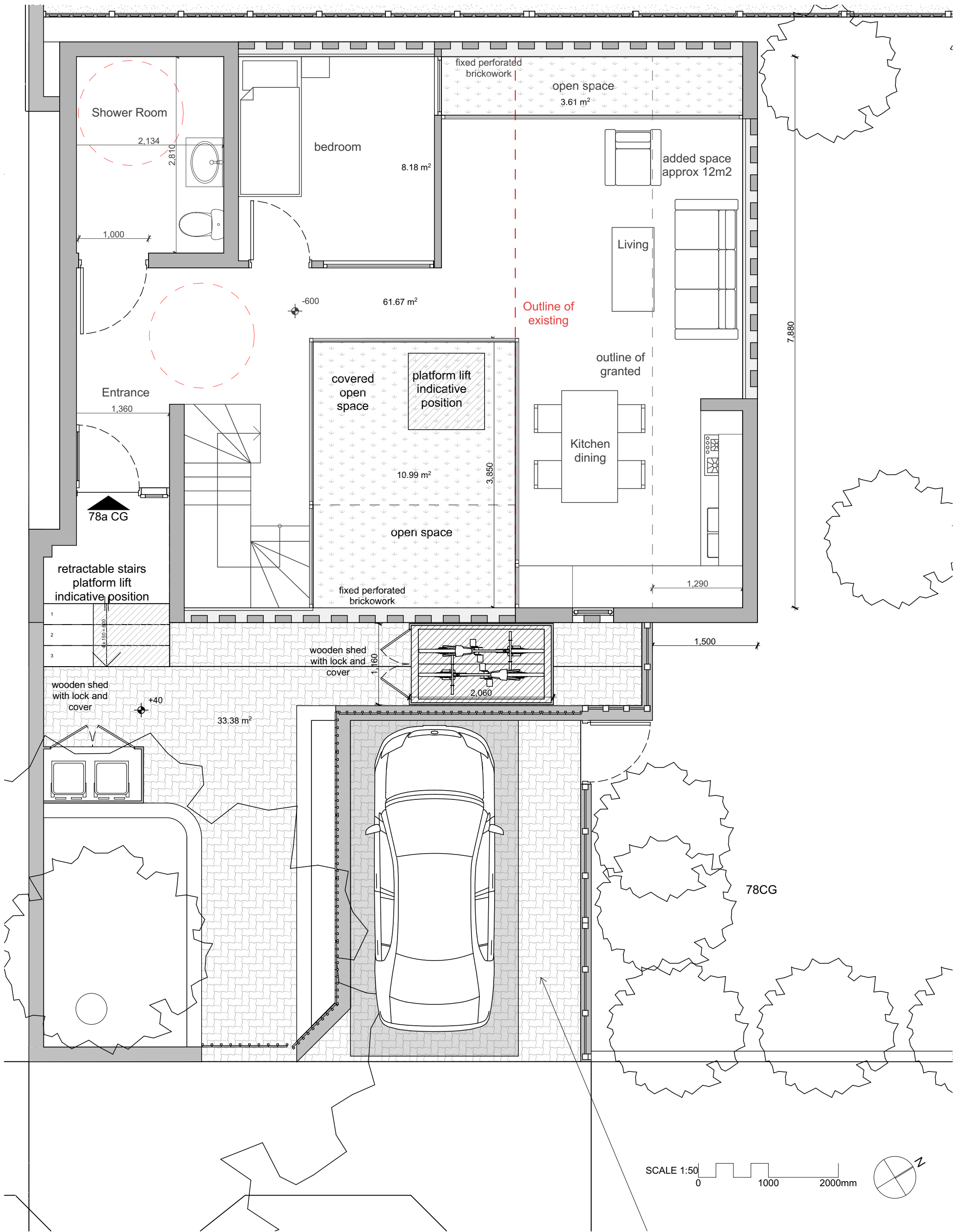
01 Proposed Ground Floor Plan
