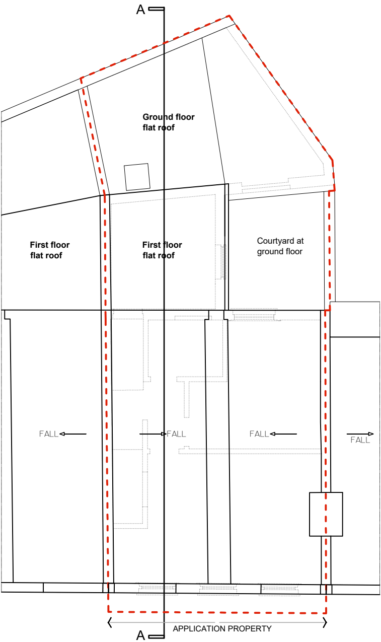
ROOF PLAN
