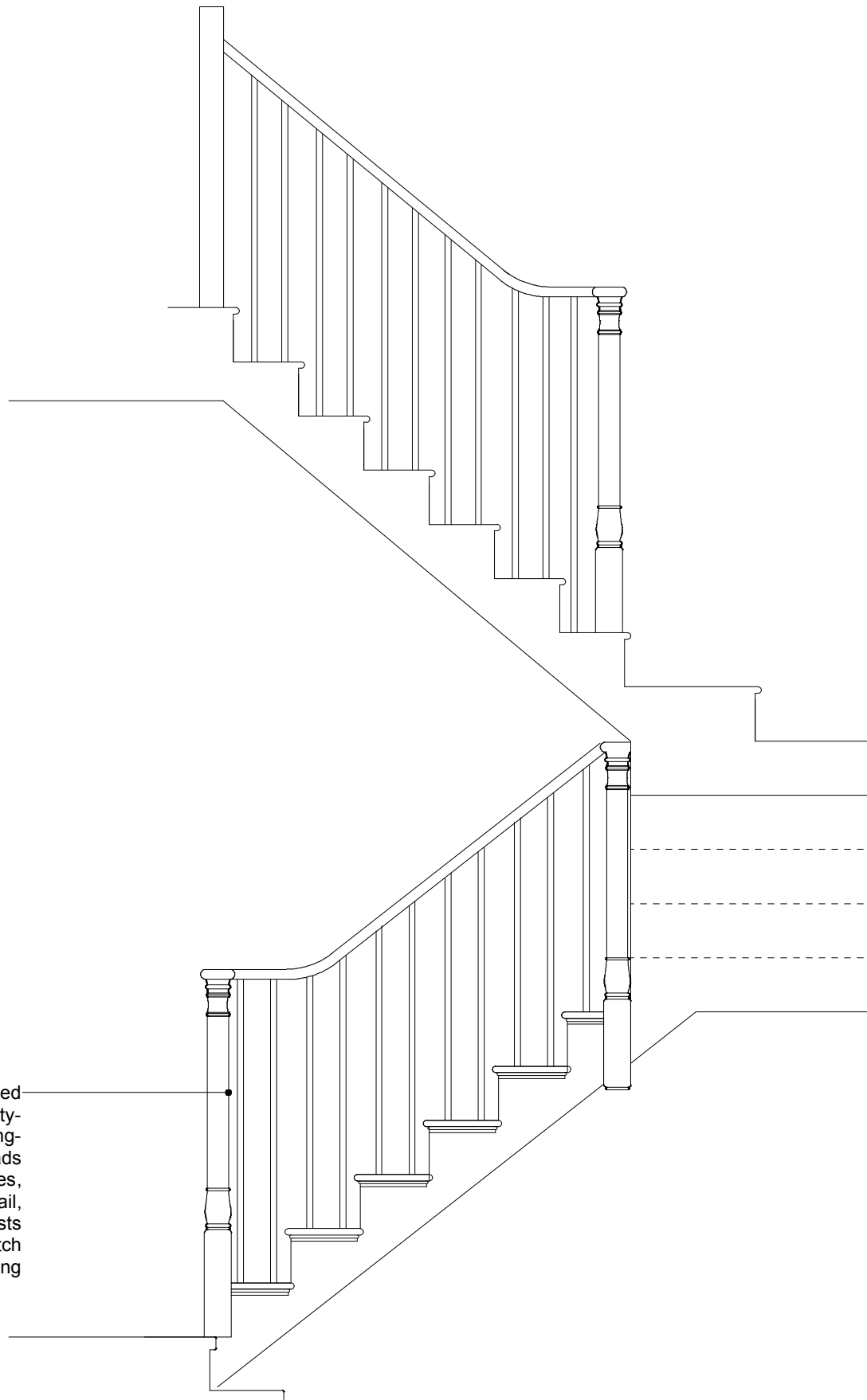
Stair Section
