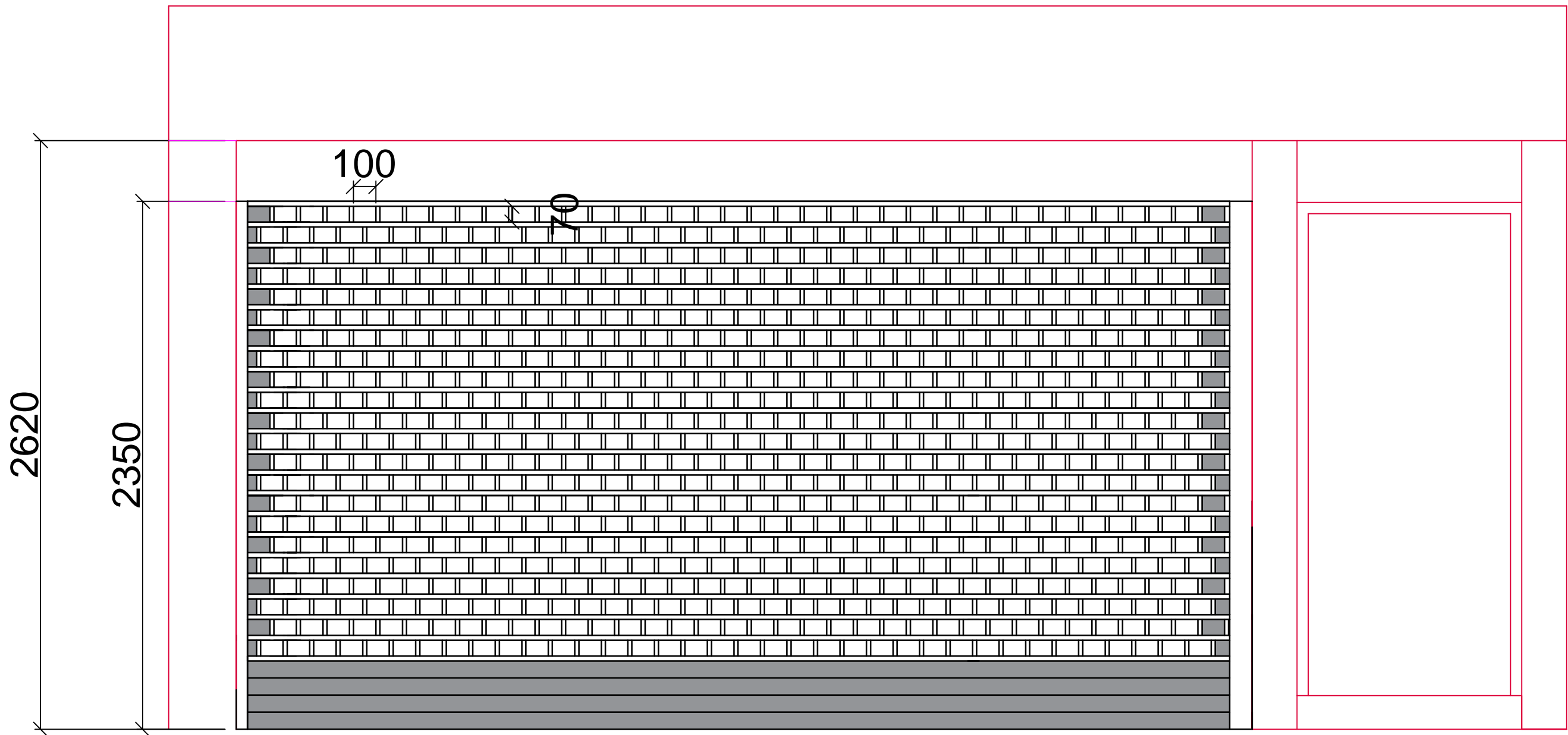
Proposed Shopfront Elevation Shutter closed
