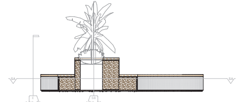
SC SEATING PLATFORM - BSMT FLOOR - SECTION C 1: 25
