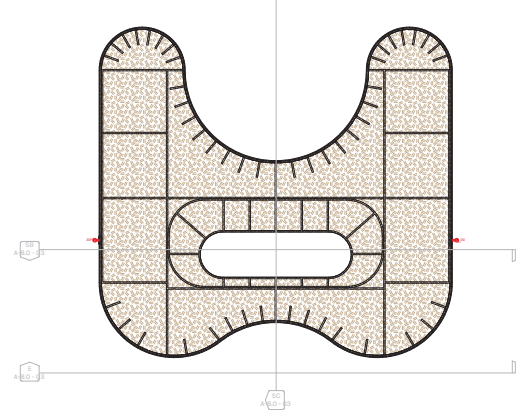
SA SEATING PLATFORM - BSMT FLOOR - SECTION A 1: 25
