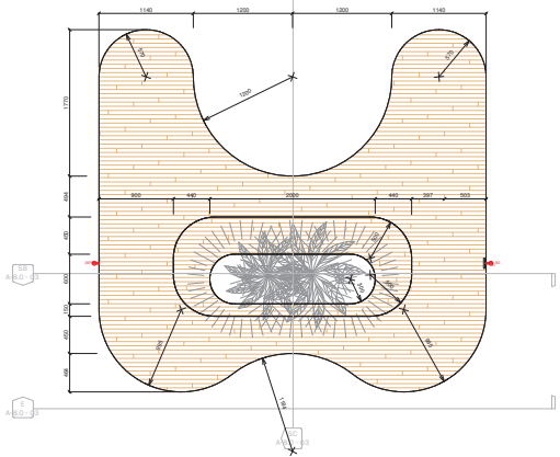
FR SEATING PLATFORM - BSMT FLOOR - FLOOR PLAN 1: 25
