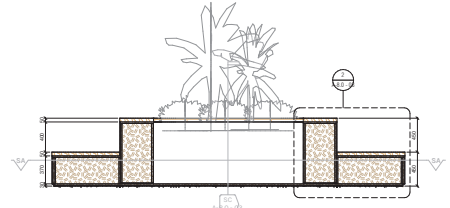
SB SEATING PLATFORM - BSMT FLOOR - SECTION B 1: 25
