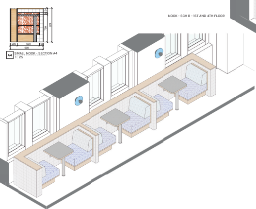
NOOK - TYPICAL - DETAIL 2
