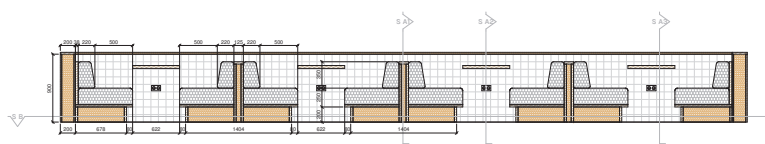
NOOK - 1ST&4TH FLOOR - ELEVATION
