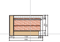
NOOK - 1ST&4TH FLOOR - SECTION 3
