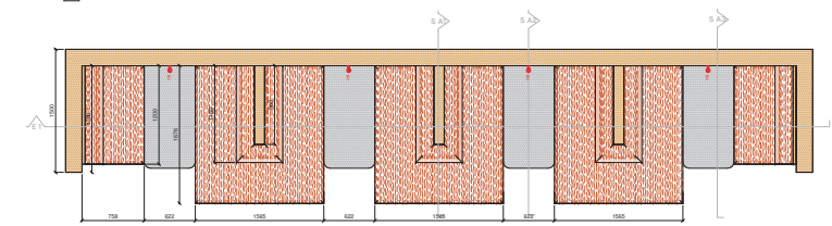
NOOK - 1ST&4TH FLOOR - FLOOR PLAN
