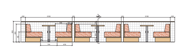
SINGLE NOOK - 1ST FLOOR - ELEVATION
