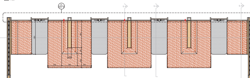
FZ NOOK - BSMNT - FLOOR PLAN 1:20
