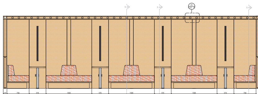
E NOOK - BSMNT FLOOR - ELEVATION 1:20
