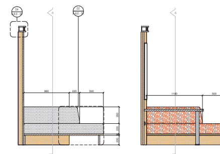
A1 NOOK - BSMNT - SECTION A1 1:20
