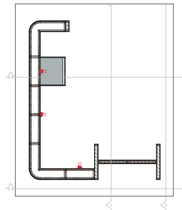
C COMMUNITY BAR - BSMT FLOOR - SECTION C 1:25
