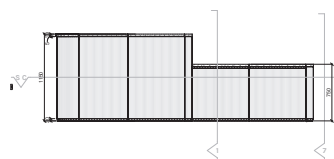
A COMMUNITY BAR - BSMT FLOOR - ELEVATION A 1:25
