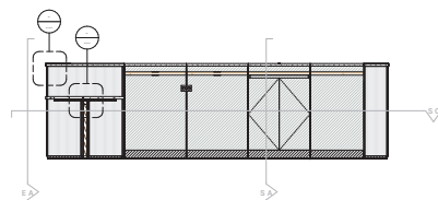
B COMMUNITY BAR - BSMT FLOOR - SECTION B 1:25
