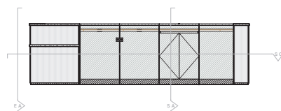
B COMMUNITY BAR - BSMT FLOOR - ELEVATION B 1:25
