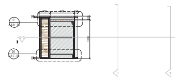
A COMMUNITY BAR - BSMT FLOOR - SECTION A 1:25
