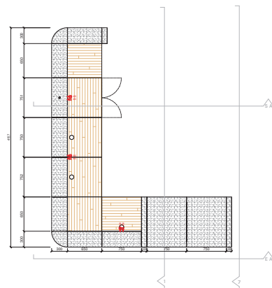
PF COMMUNITY BAR - BSMT FLOOR - FLOOR PLAN 1:25
