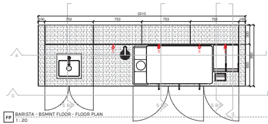
FP BARISTA - BSMT FLOOR - FLOOR PLAN 1:20
