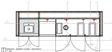
3 BARISTA - BSMT FLOOR - SECTION C 1:20
