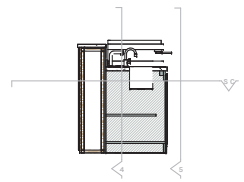
82 BARISTA - BSMT FLOOR - SECTION B2 1:20
