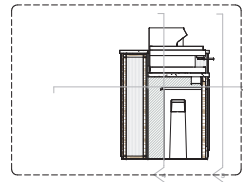
81 BARISTA - BSMT FLOOR - SECTION B1 1:20
