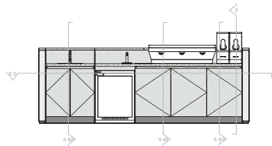
1 BARISTA - BSMT FLOOR - ELEVATION 1:20
