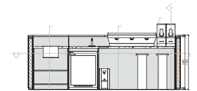
4 BARISTA - BSMT FLOOR - SECTION A 1:20
