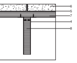
5 Detail 5 1:5
