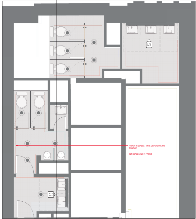
1 PL-RESTROOMS.2 1:25
