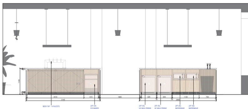
BE BSMT FL - PANTRY BACK ELEVATION 1: 25
