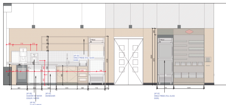
FE BSMT FL - PANTRY FRONT ELEVATION 1: 25
