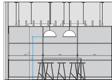
FE BRAINSTORM - BASEMENT - FRONT ELEVATION 1:25
