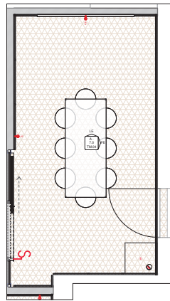
FP BRAINSTORM - BASEMENT - FLOOR PLAN 1:25
