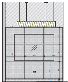
LE BRAINSTORM - BASEMENT - LEFT ELEVATION 1:25
