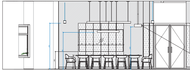
BE BOARD ROOM - BASEMENT - BACK ELEVATION 1:50
