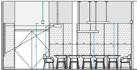
BE BOARD ROOM - BASEMENT - BACK ELEVATION 1:50
