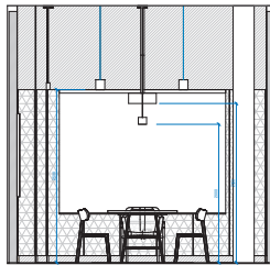
LE BOARD ROOM - BASEMENT - LEFT ELEVATION 1:50
