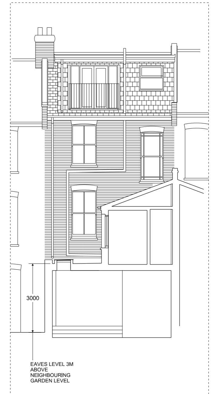
02 PROPOSED SECTION BB A2100 1:100 @ A3
