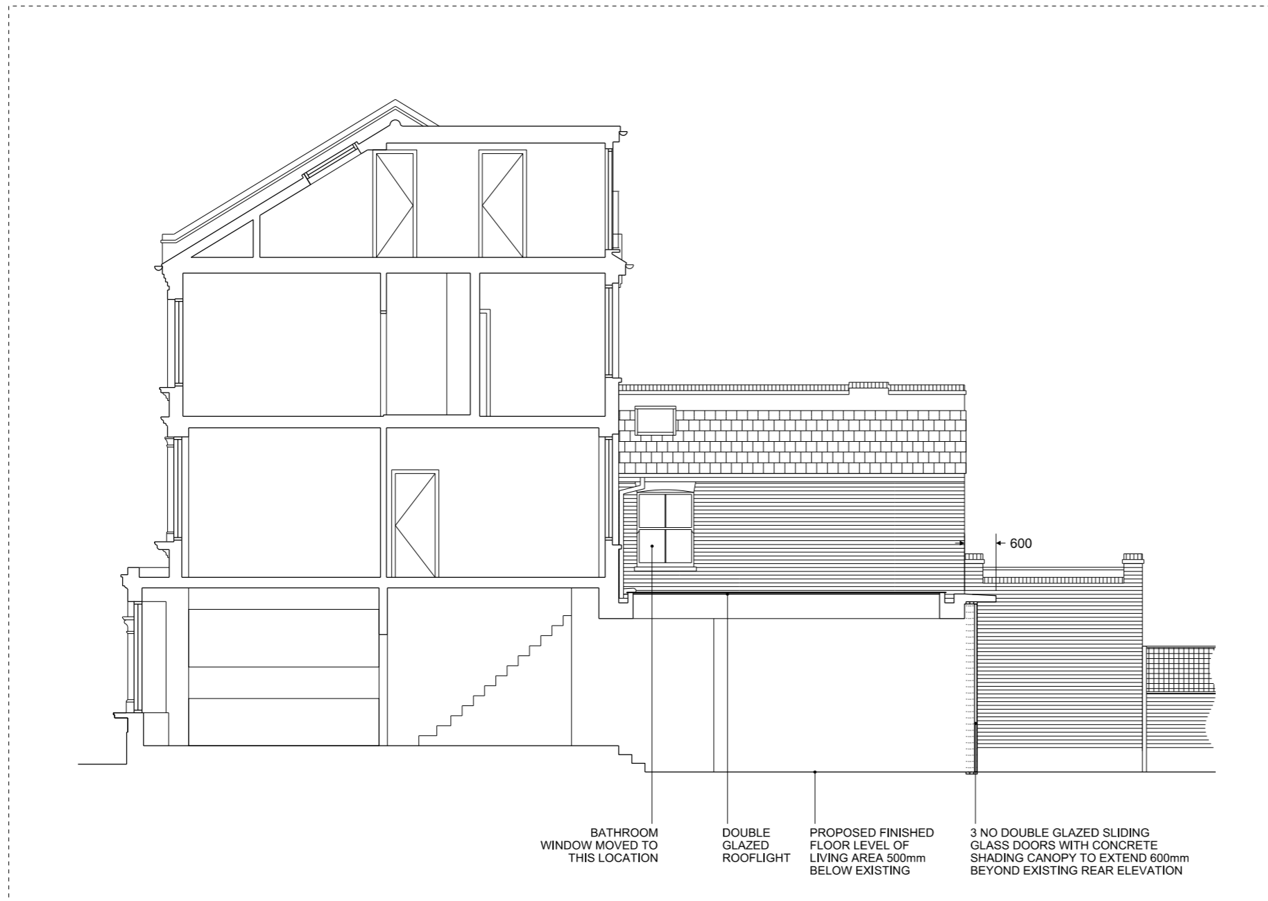
01 PROPOSED SECTION AA A2100 1:100 @ A3
