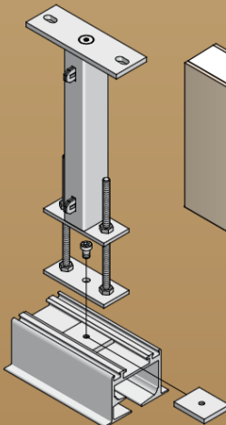
Sectional track drawing showing bracket suspension
