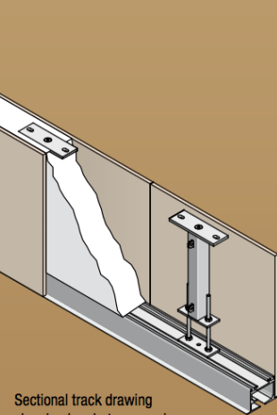
Sectional track drawing showing bracket suspension with acoustic baffle/barrier
