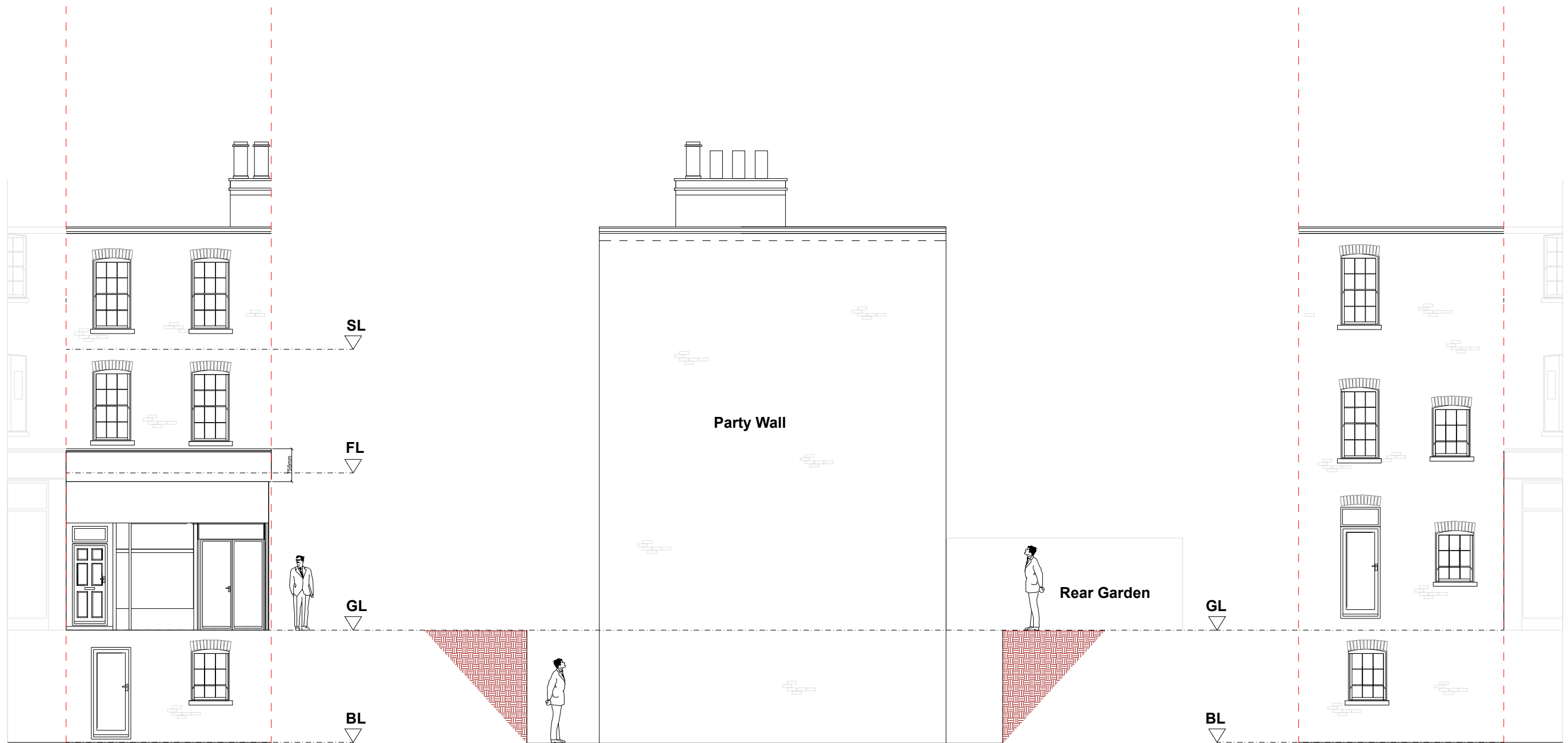
Existing Front Elevation Scale 1:100
