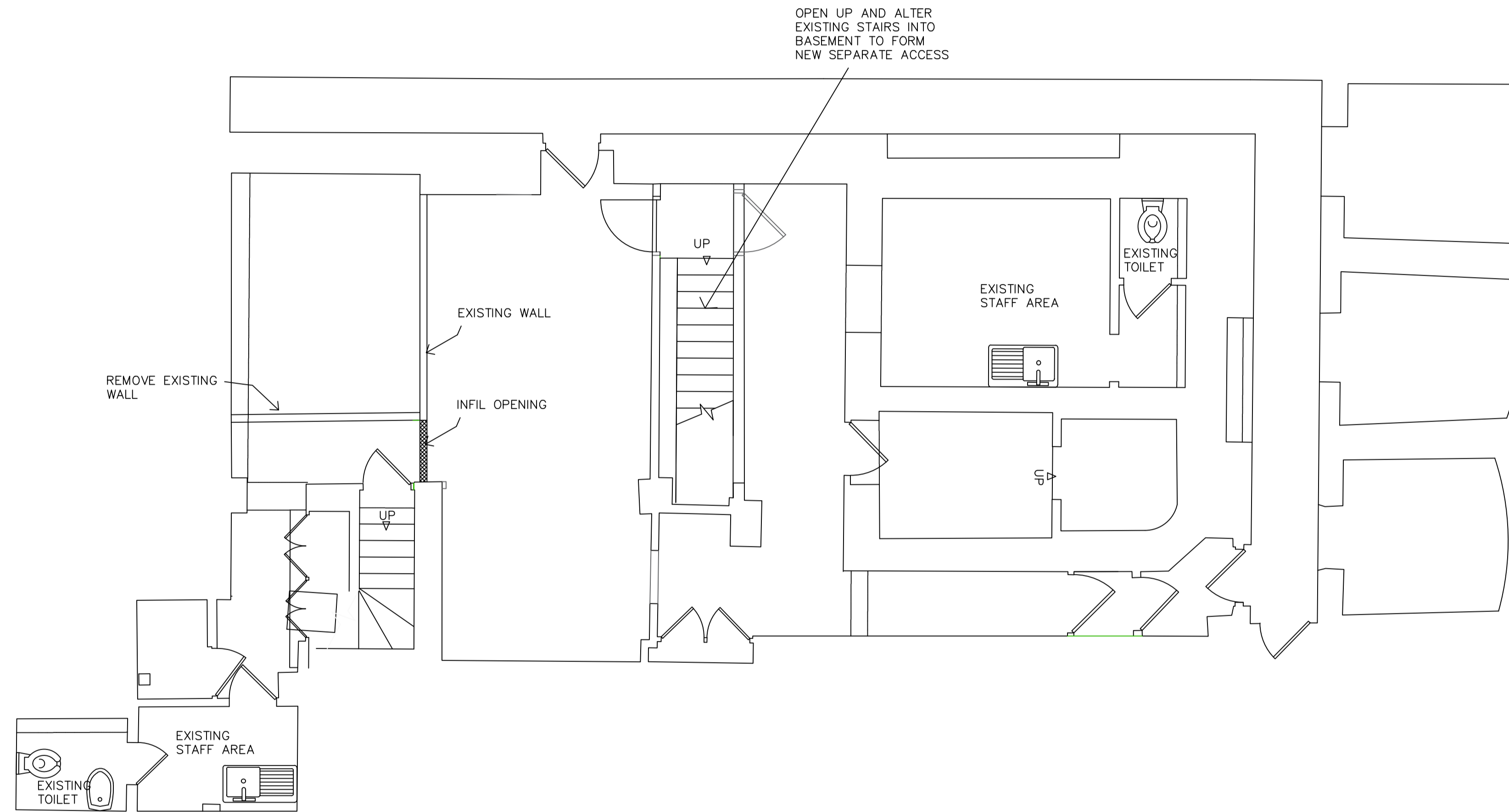
PROPOSED BASEMENT PLAN
