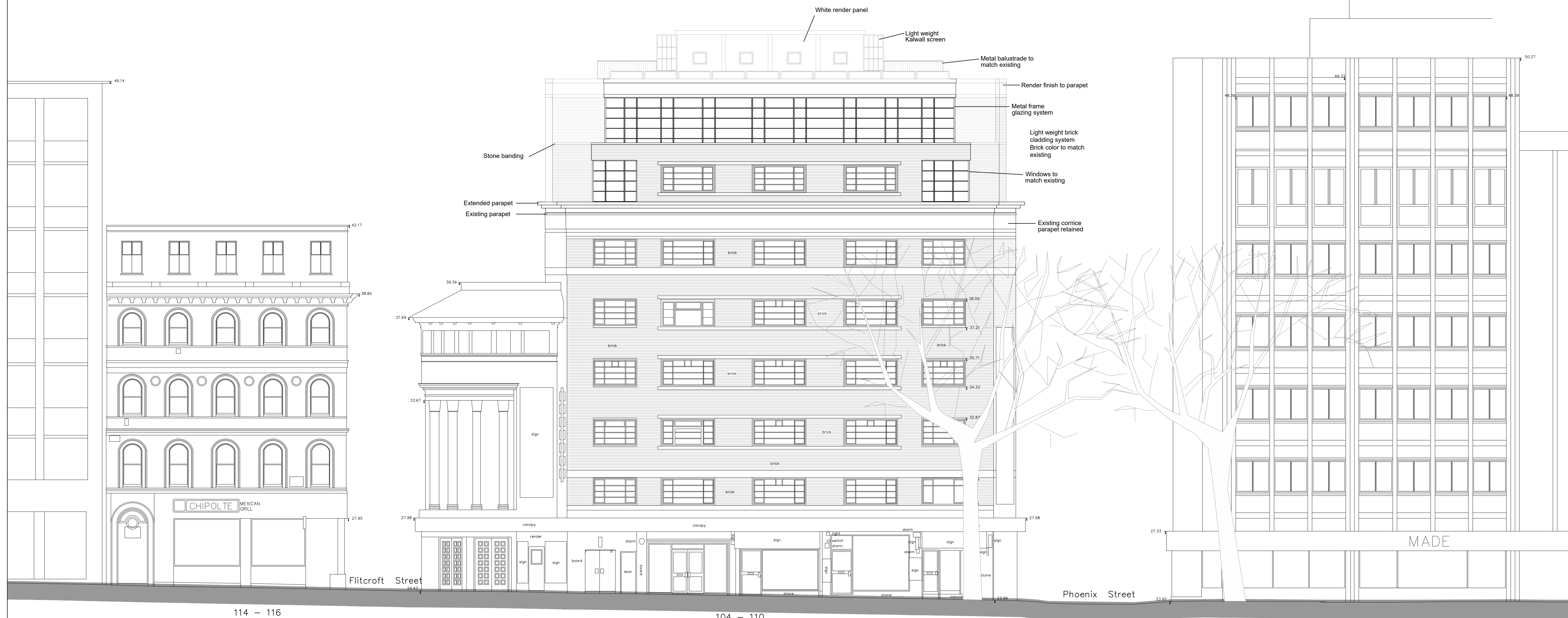
WEST ELEVATION CHARING CROSS ROAD
