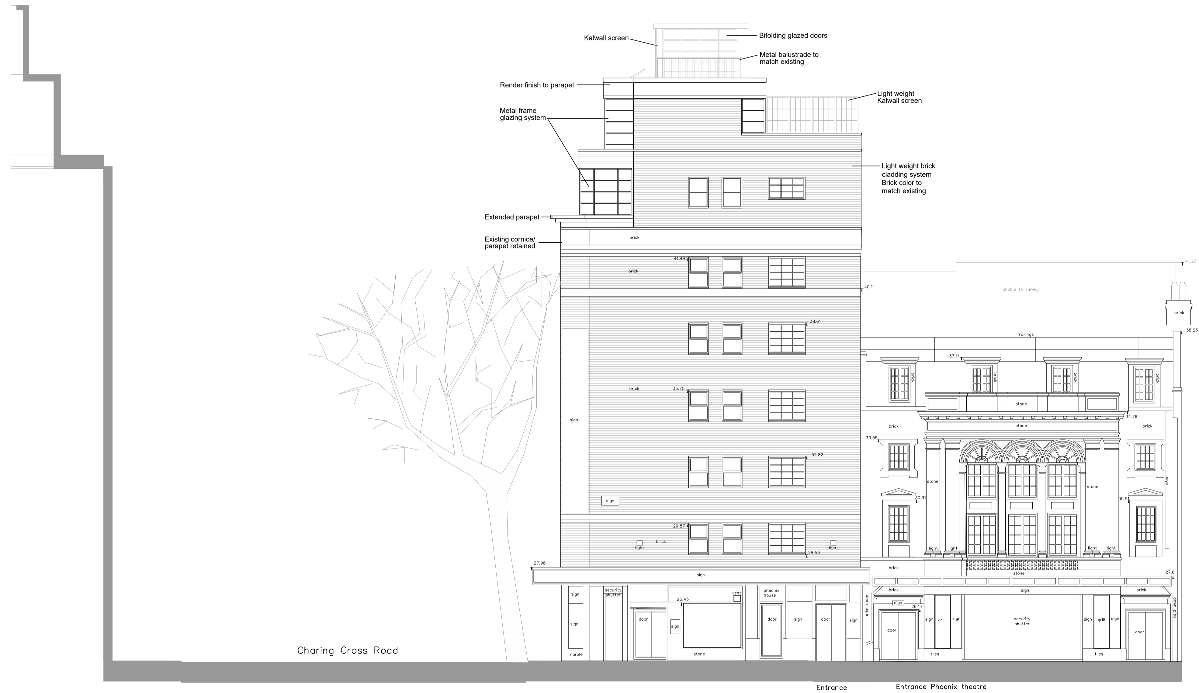
SOUTH ELEVATION PHOENIX STREET
