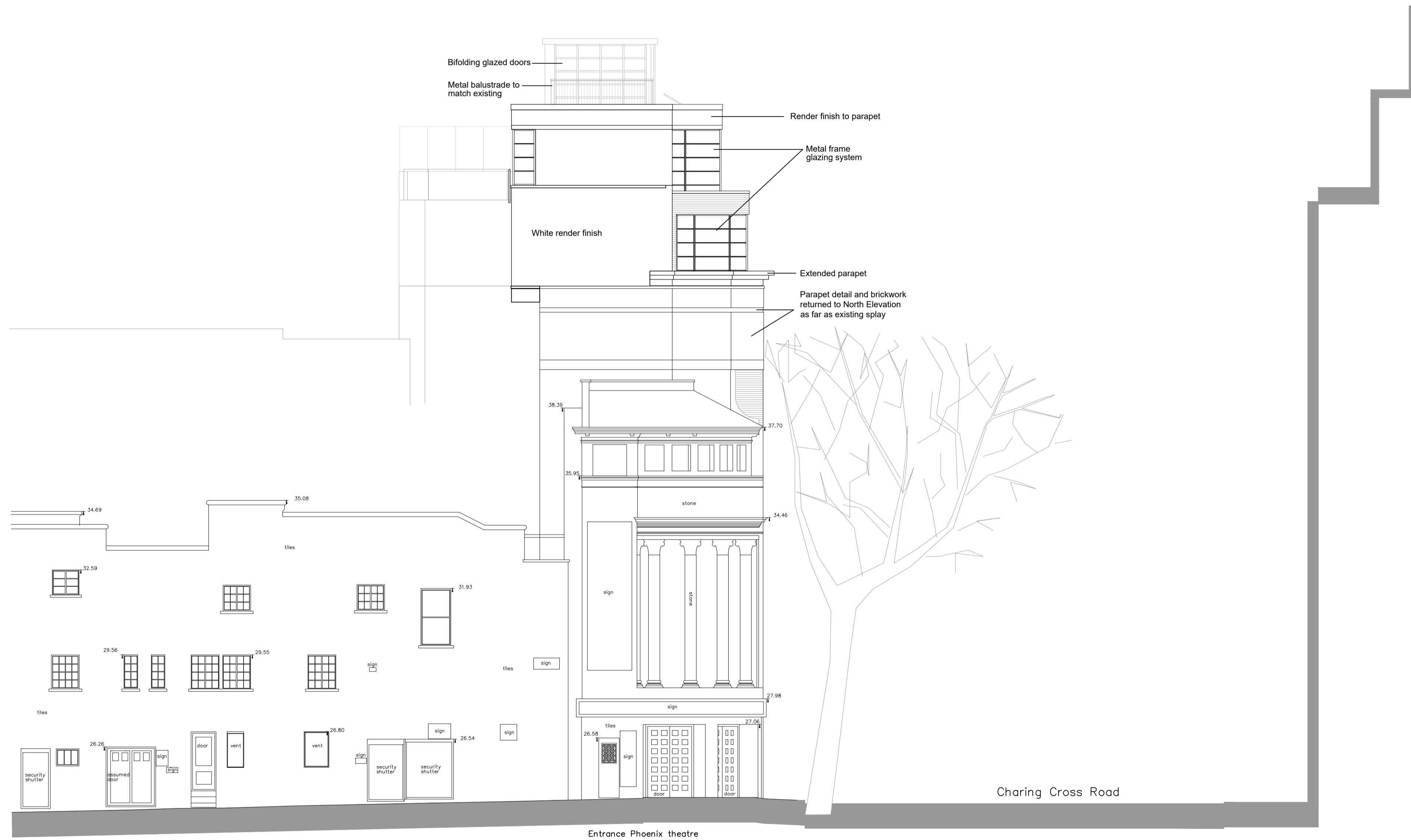
NORTH ELEVATION FLITCROFT STREET
