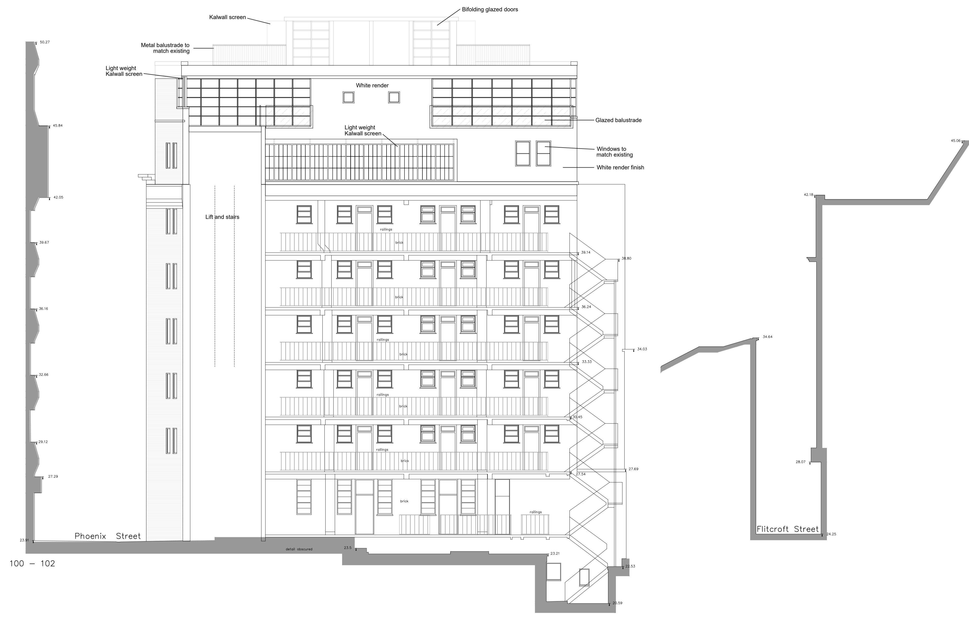
EAST REAR ELEVATION
