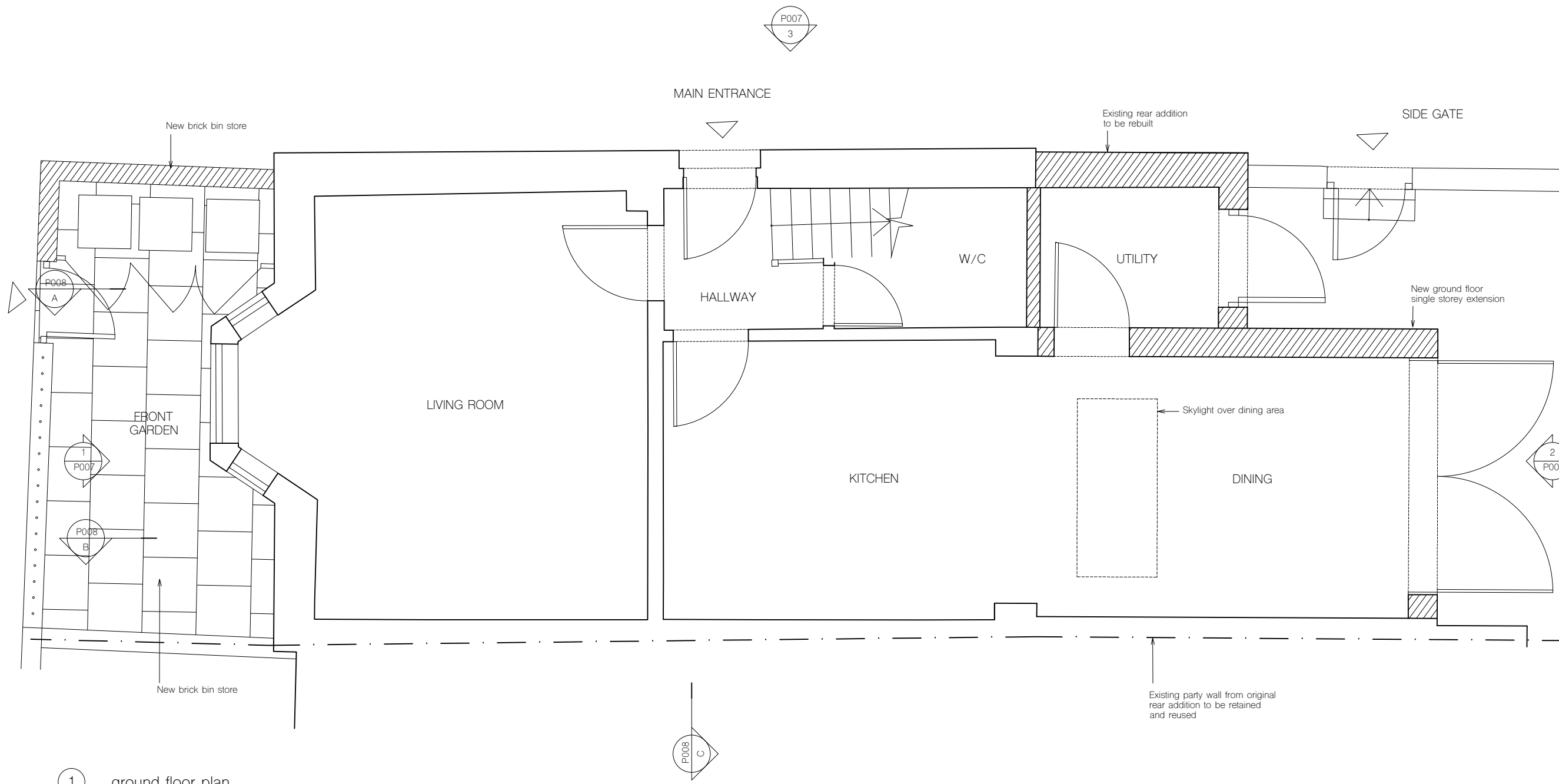
1 ground floor plan
