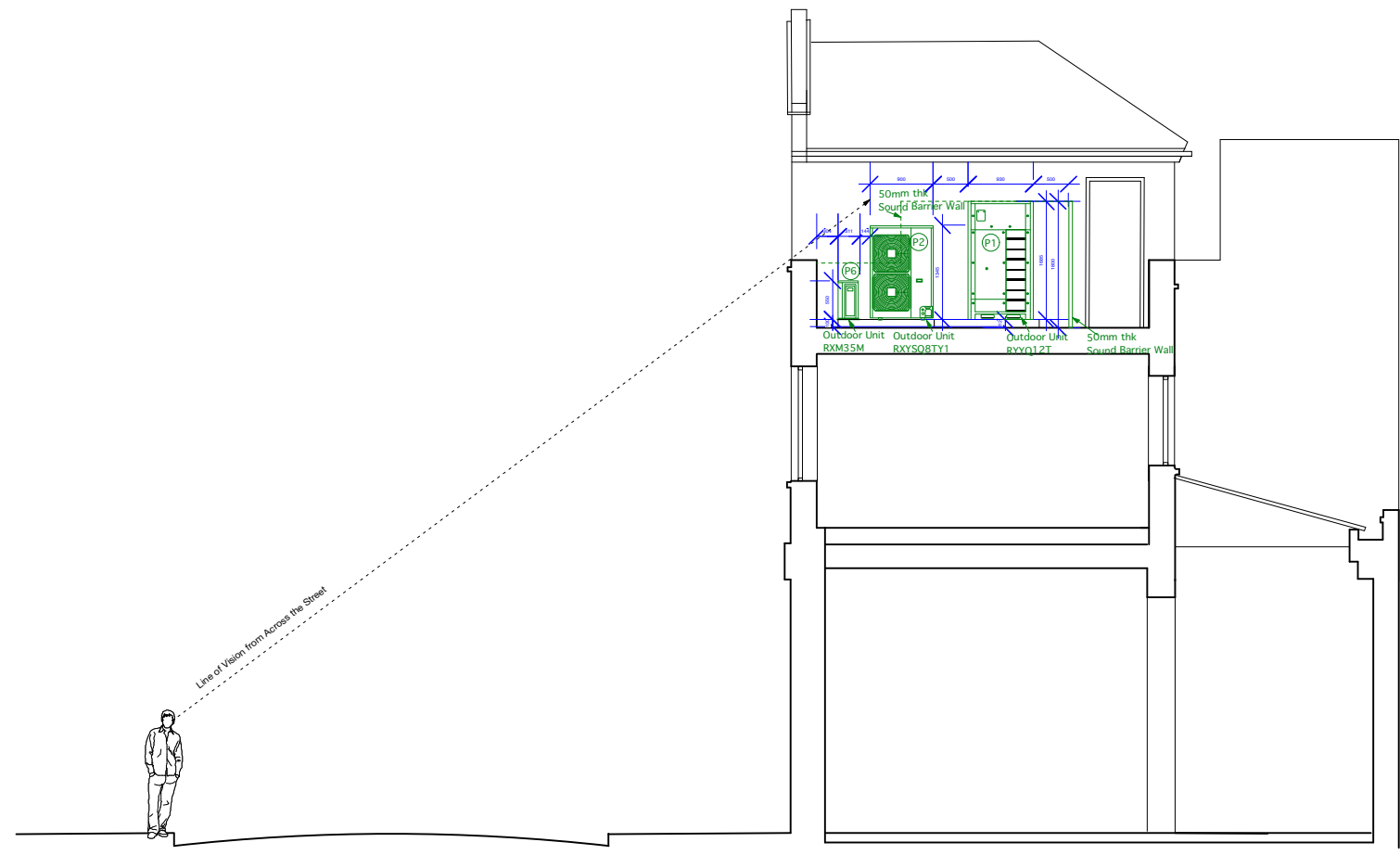
SECTION B-B
