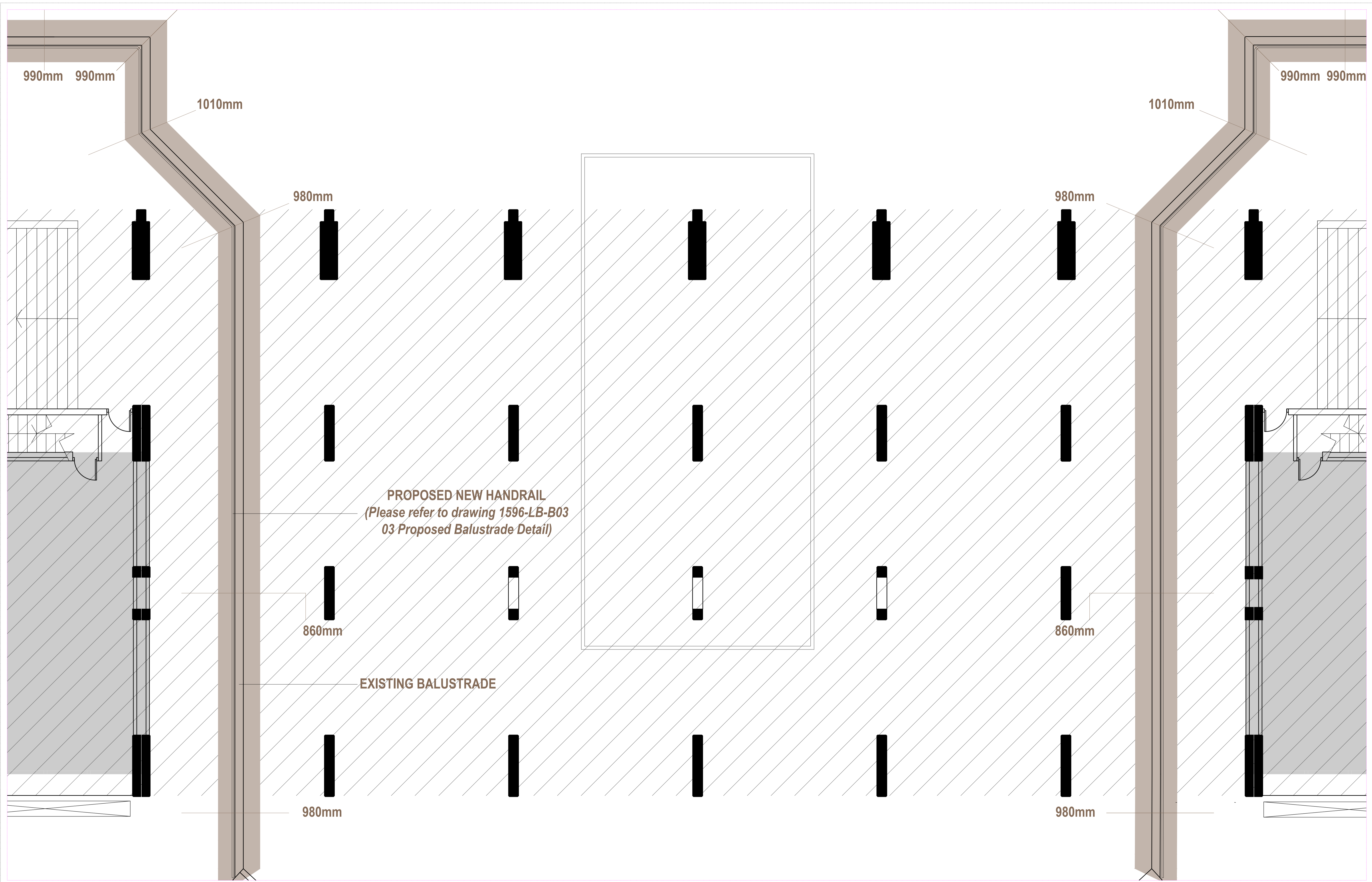
[01] PROPOSED LEVEL C (PODIUM) ENLARGED PLAN - PROPOSED BALUSTRADE HEIGHTS
