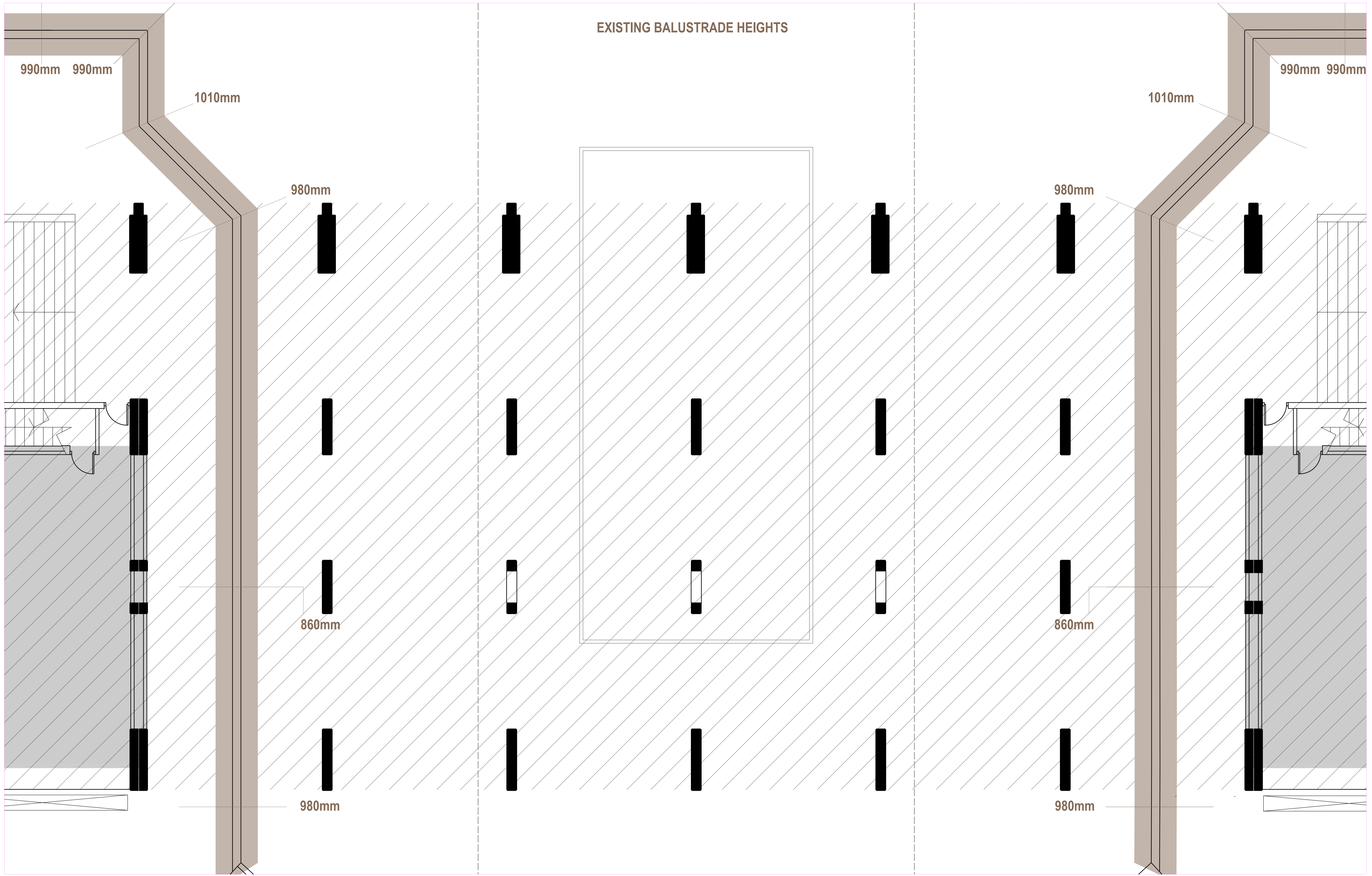
[01] EXISTING LEVEL C (PODIUM) ENLARGED PLAN - EXISTING BALUSTRADE HEIGHTS
