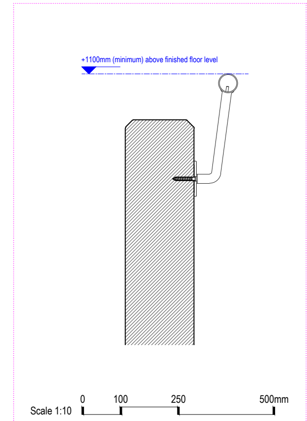
[04] PROPOSED BALUSTRE DETAIL S:1/10
