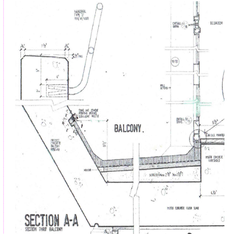
[06] PRECEDENT DETAIL (BRUNSWICK FLATS BALUSTRADE) S: 1/10
