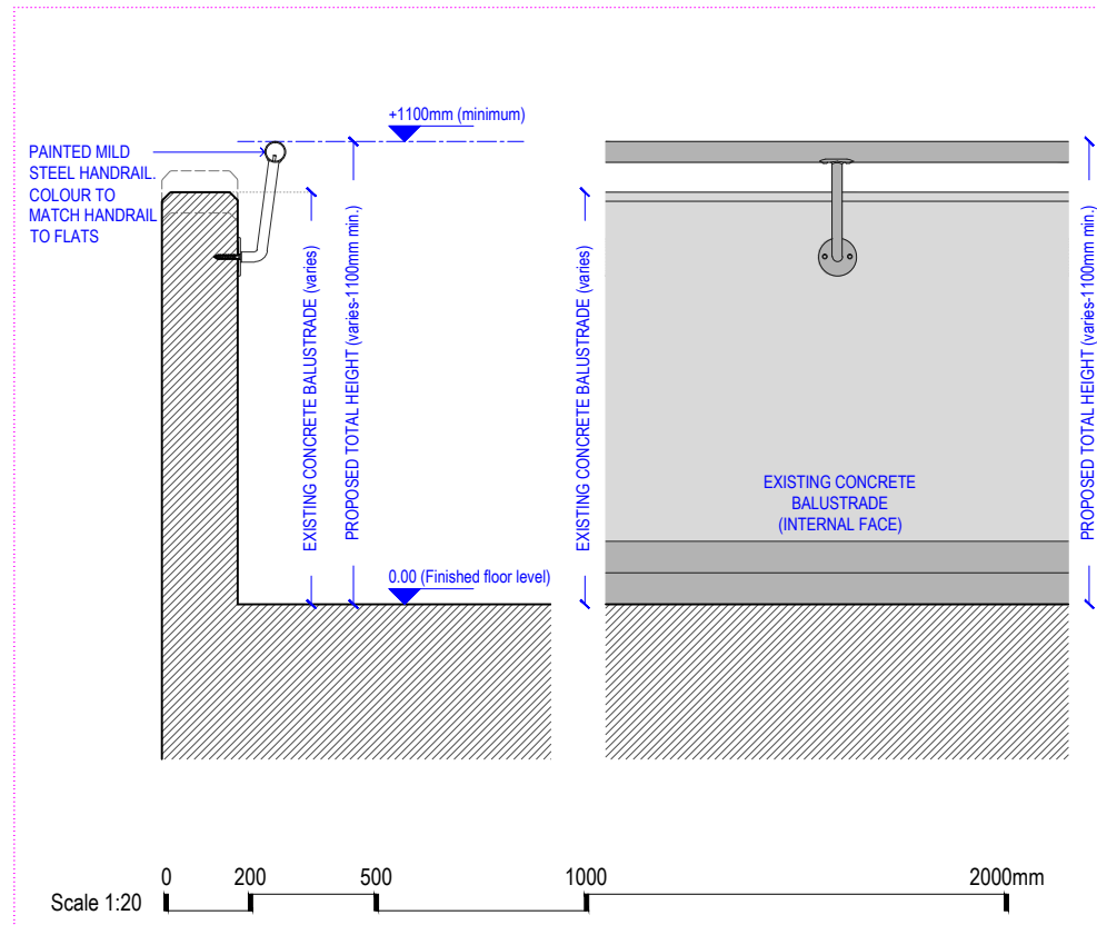
[03] PROPOSED BALUSTRE DETAIL S:1/20
