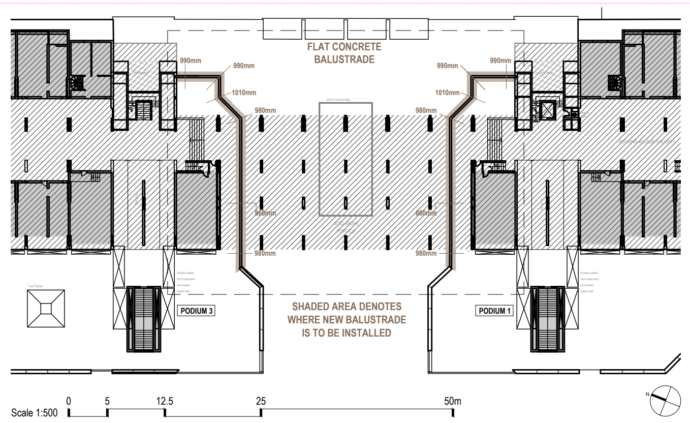
[01] EXISTING LEVEL C (PODIUM) FLOOR PLAN - EXISTING BALUSTRADE HEIGHTS FROM FINISHED FLOOR LEVEL S:1/500
