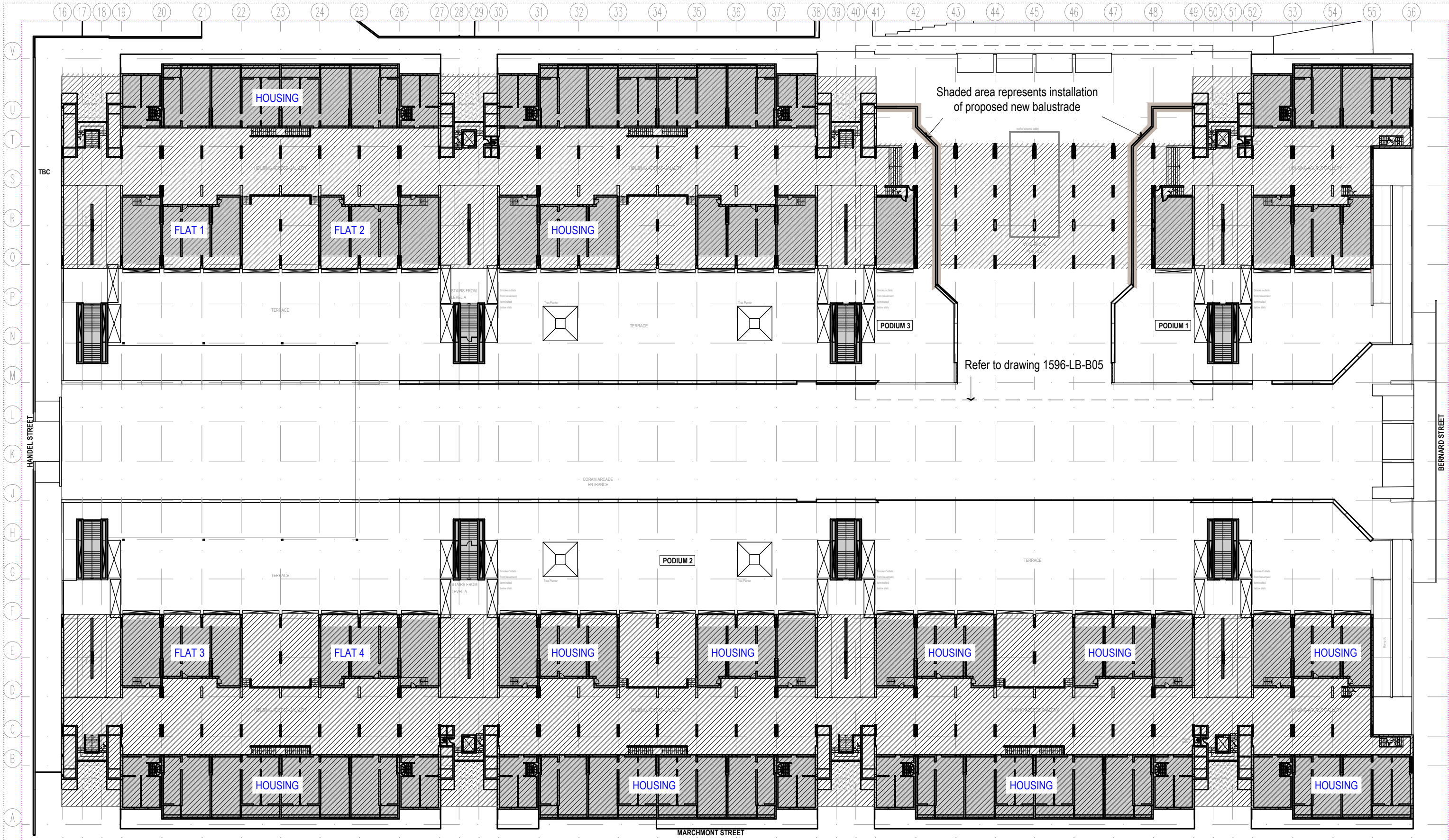
[01] EXISTING LEVEL C (PODIUM) BLOCK PLAN
