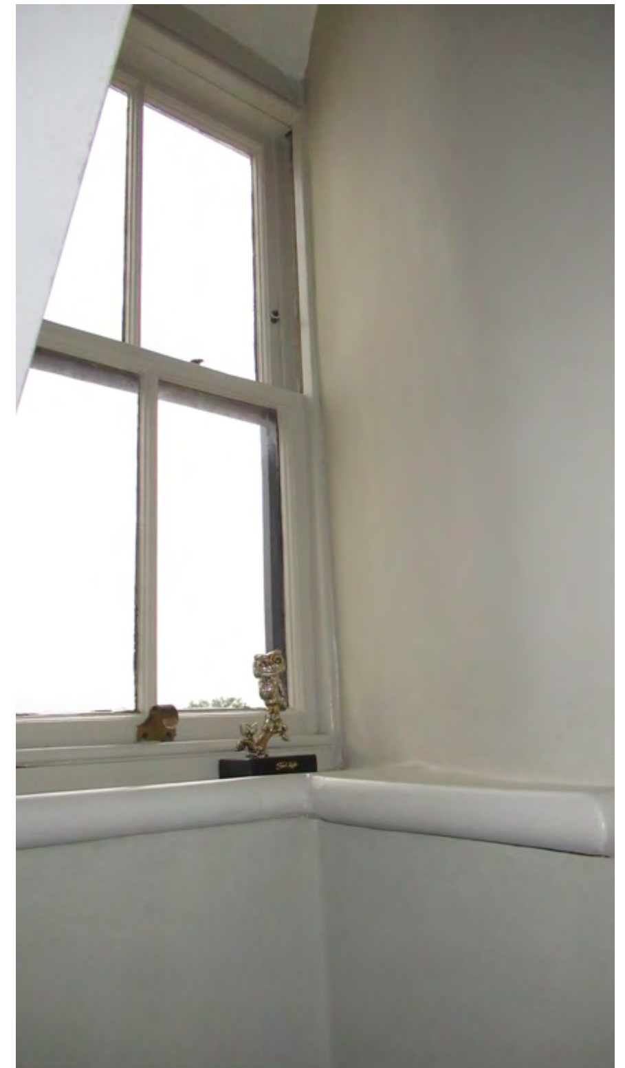
Figure 14: View showing the junction between the existing sash window and internal dividing wall. Secondary glazing will be supported on the existing cill and attached to the window jambs
