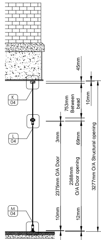
Section View B:B @ 1:50
