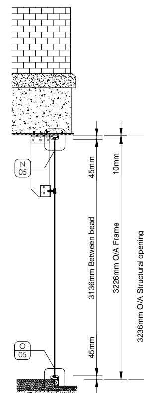
Section View C:C @ 1:50
