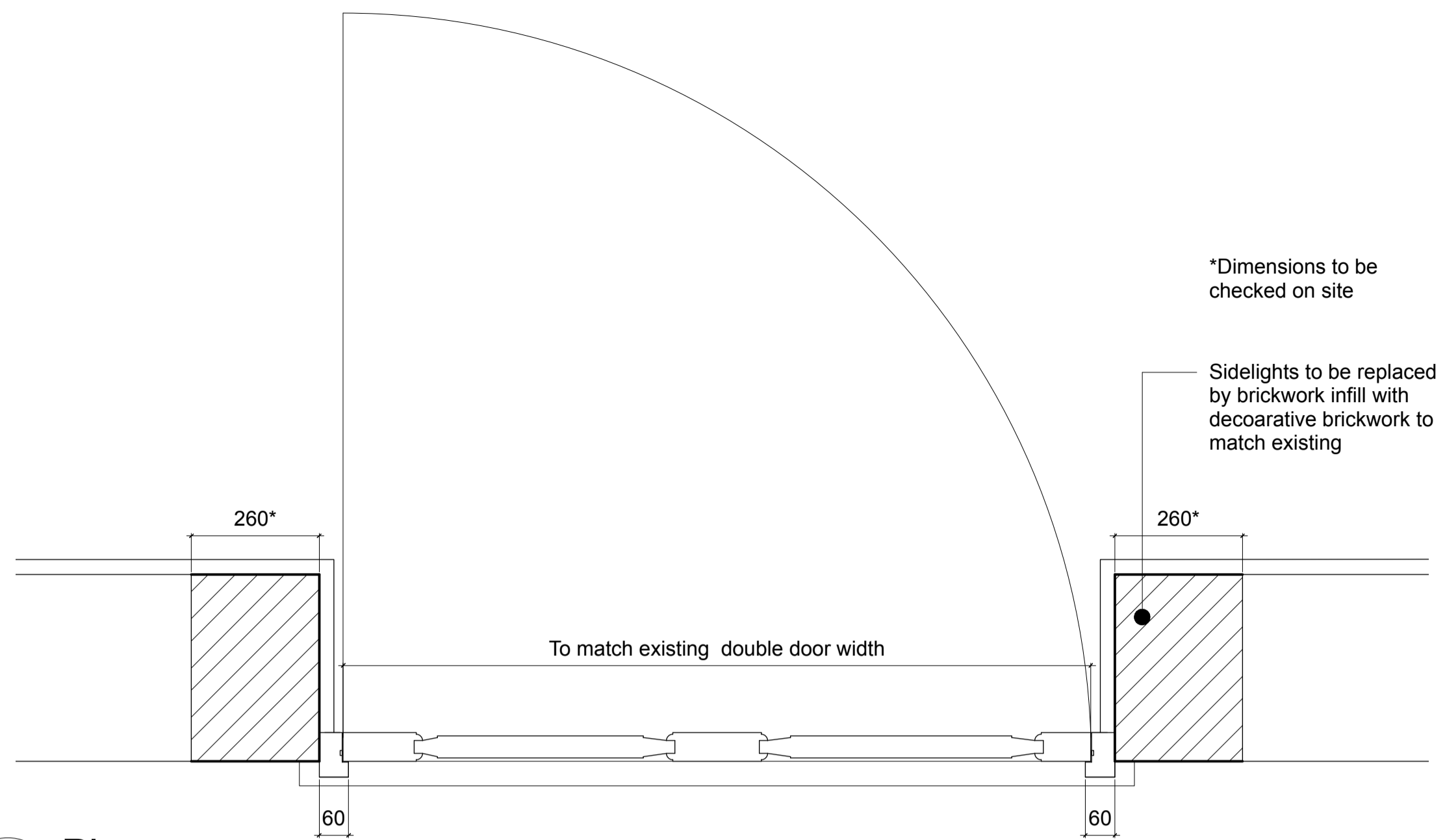
1 Plan 1:10 @ A1
