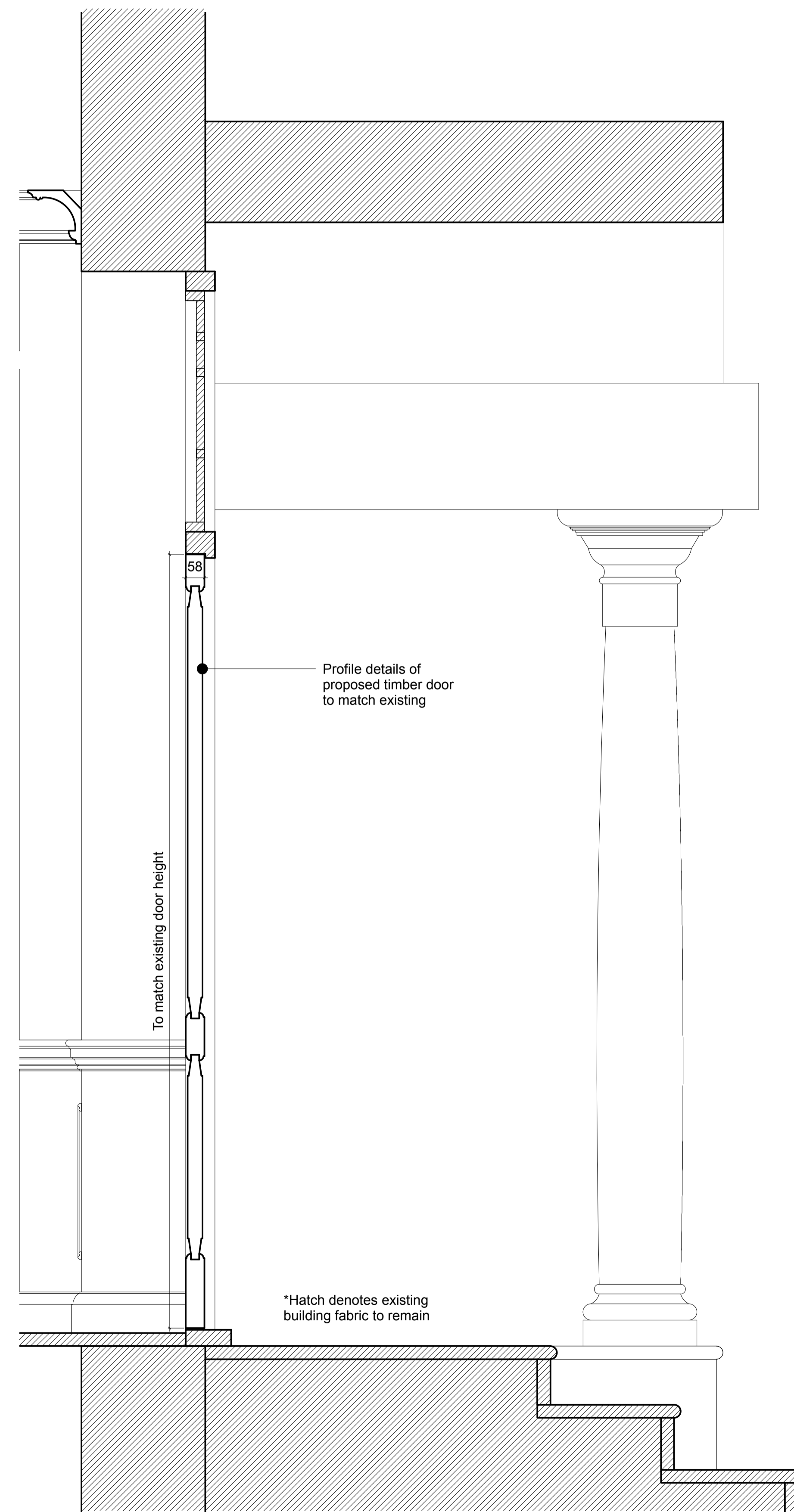
3 Section 1:10 @ A1
