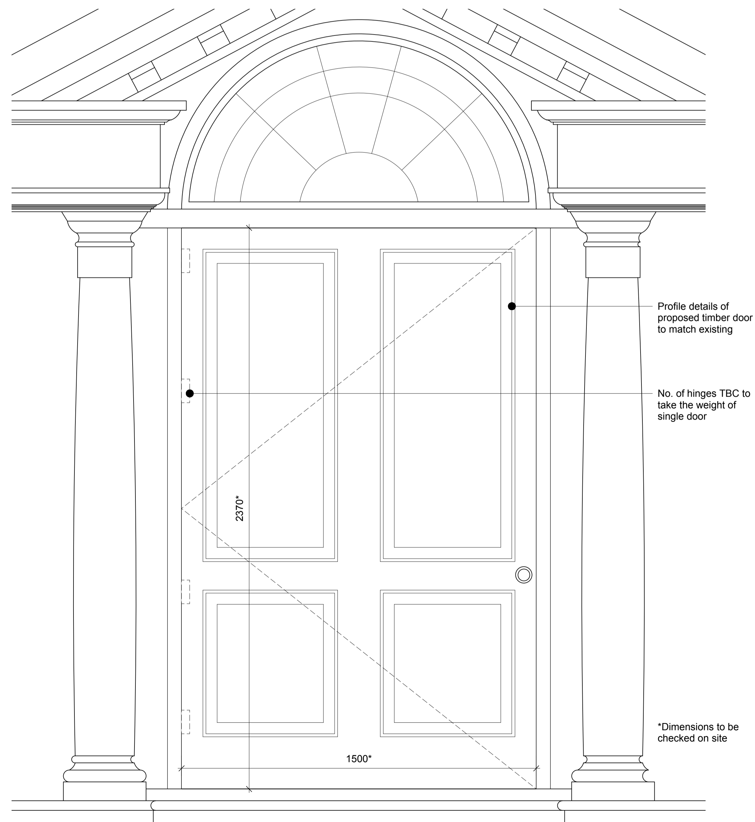
2 Elevation 1:10 @ A1
