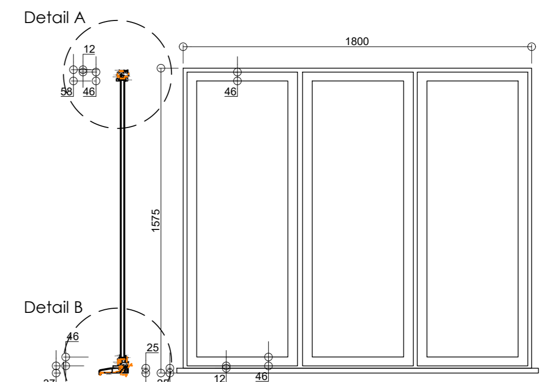
Window sectional detail Alitherm Heritage casements Scale 1:20
