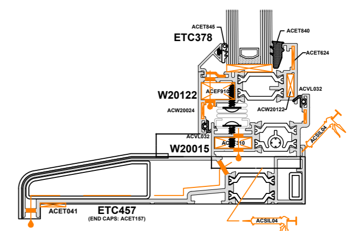
Detail B: Cill detail 1:2
